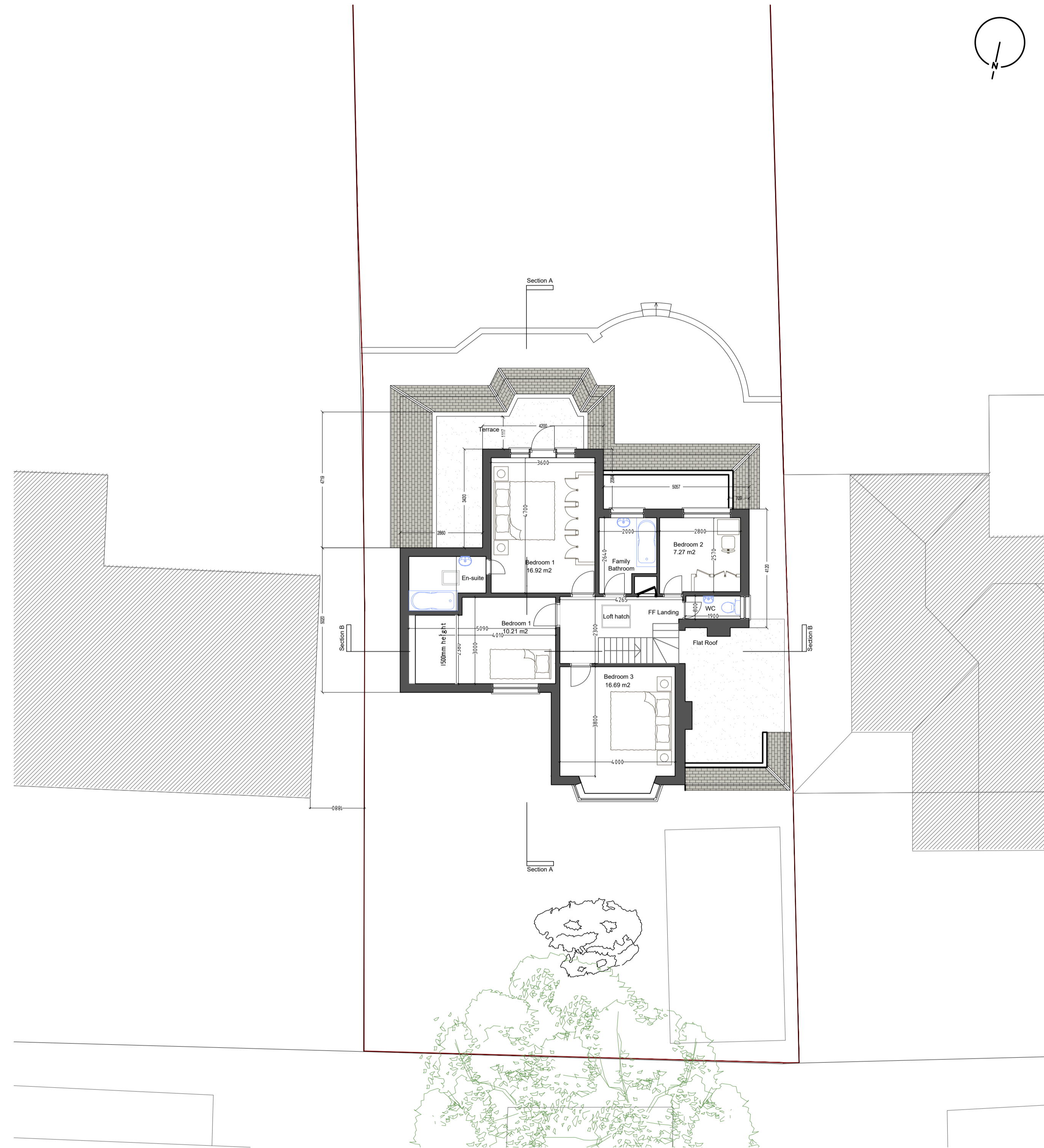
scale 1:100 0m 1m 2m 3m 4m 5m First Floor Plan - Existing
