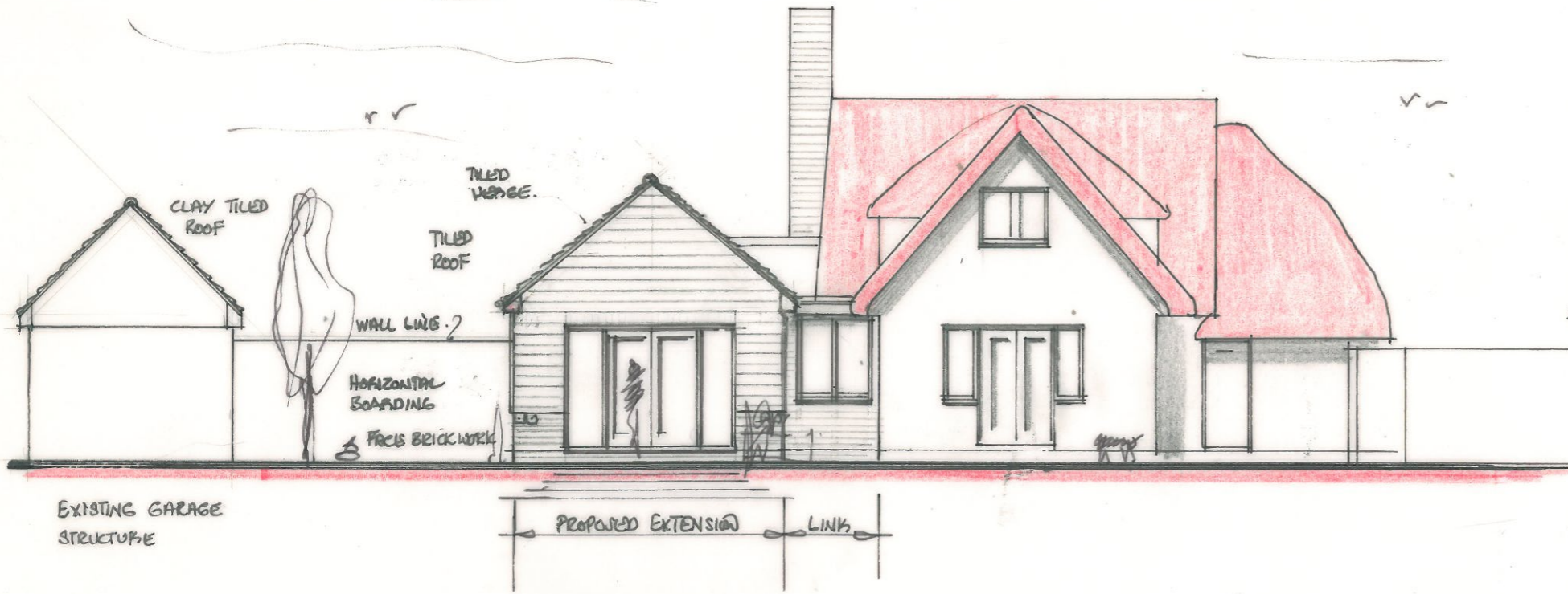
REAR ELEVATION.
