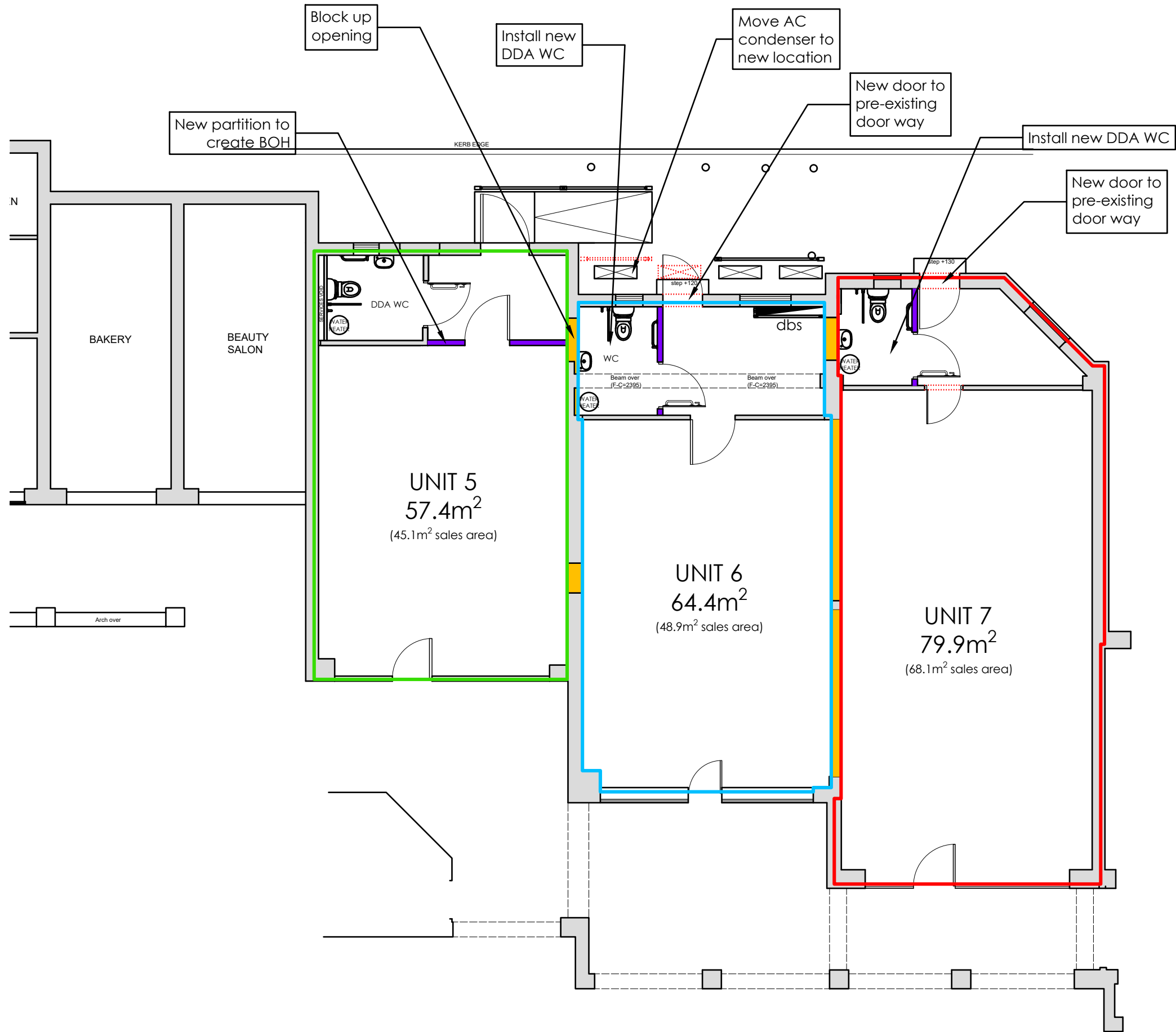
① Ground Floor Plan Scale 1:100
