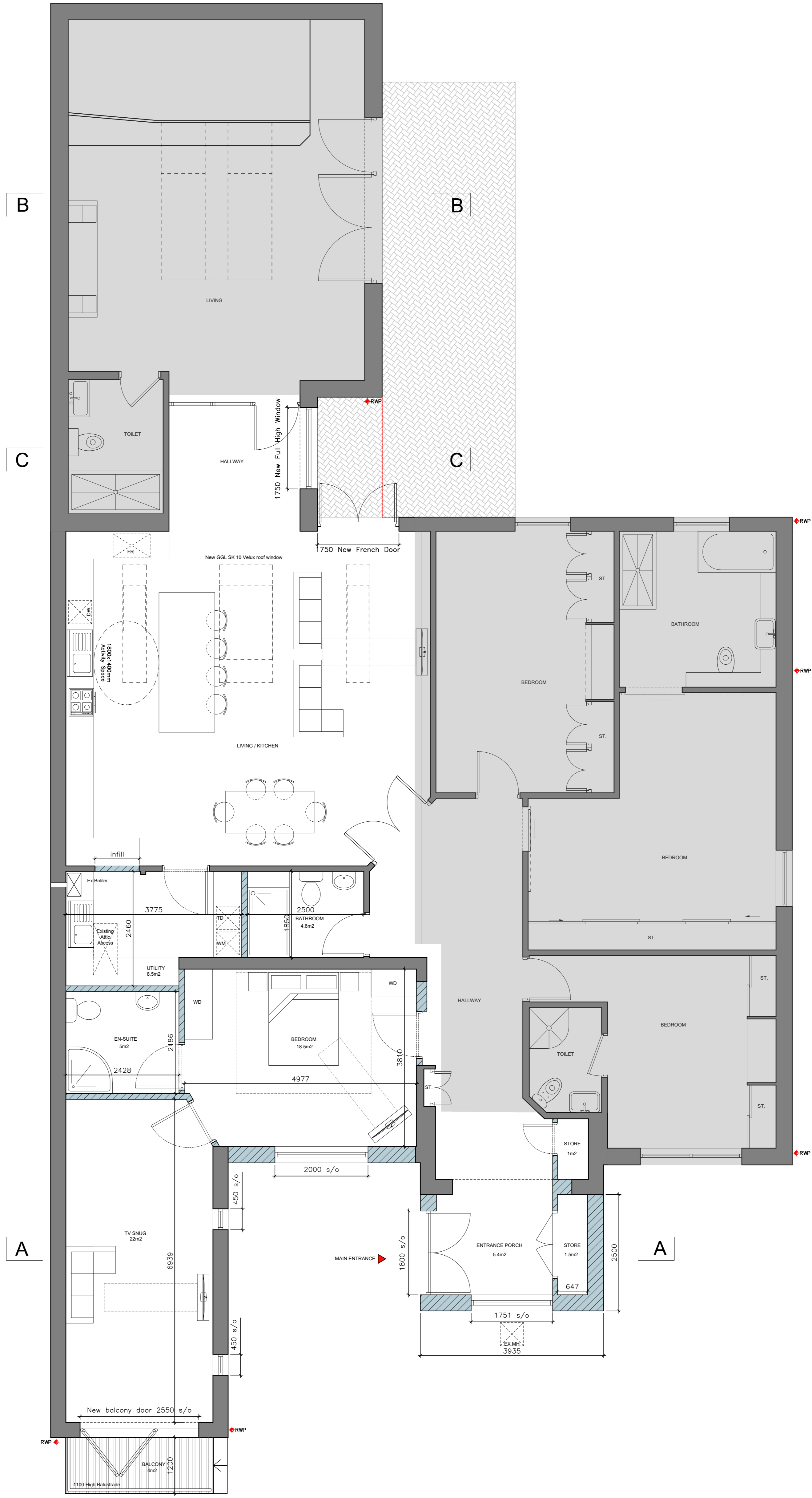
Proposed Ground Floor Plan 1:50 0 5m
