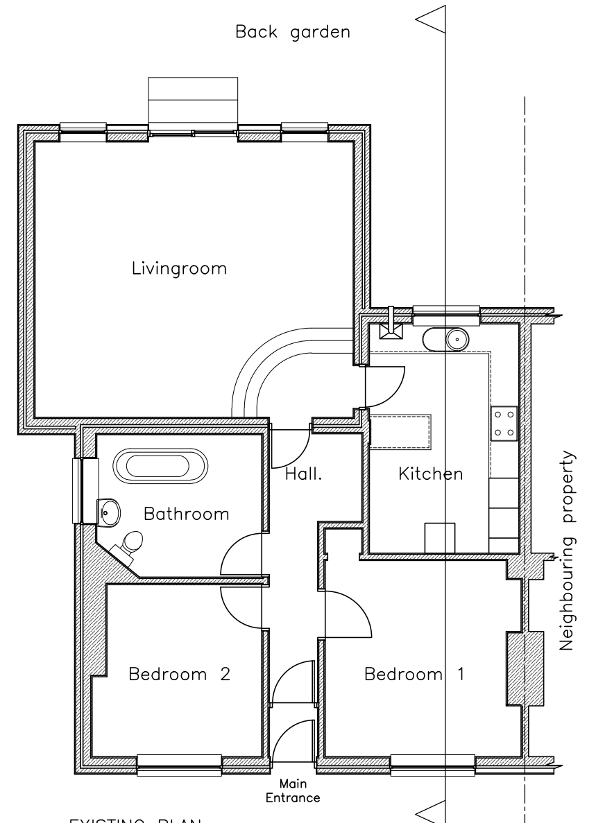
EXISTING PLAN. SCALE 1:100.
