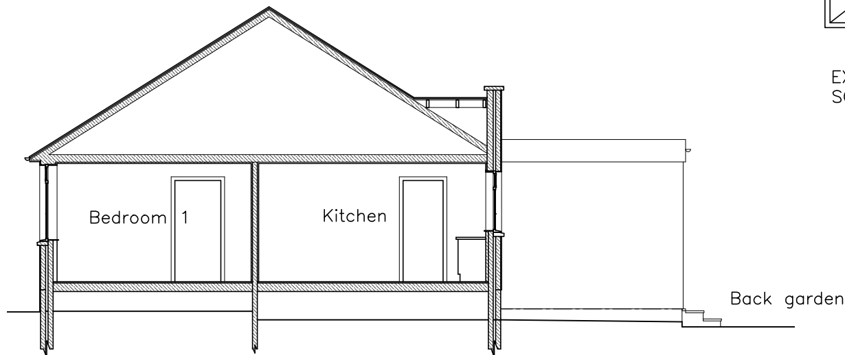
EXISTING SECTION / SIDE ELEVATION. SCALE 1:100.
