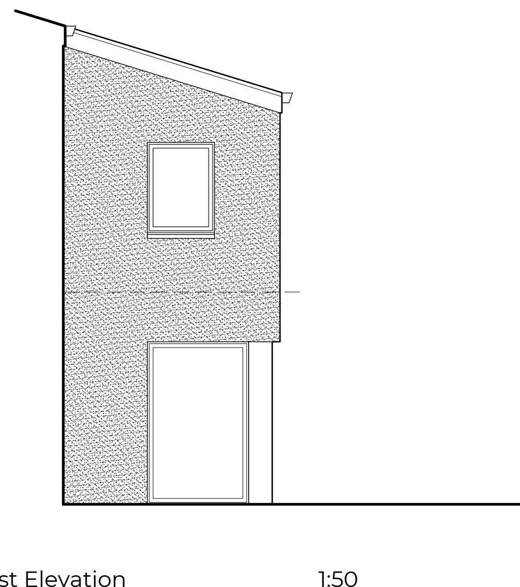
Partial West Elevation 1:50
