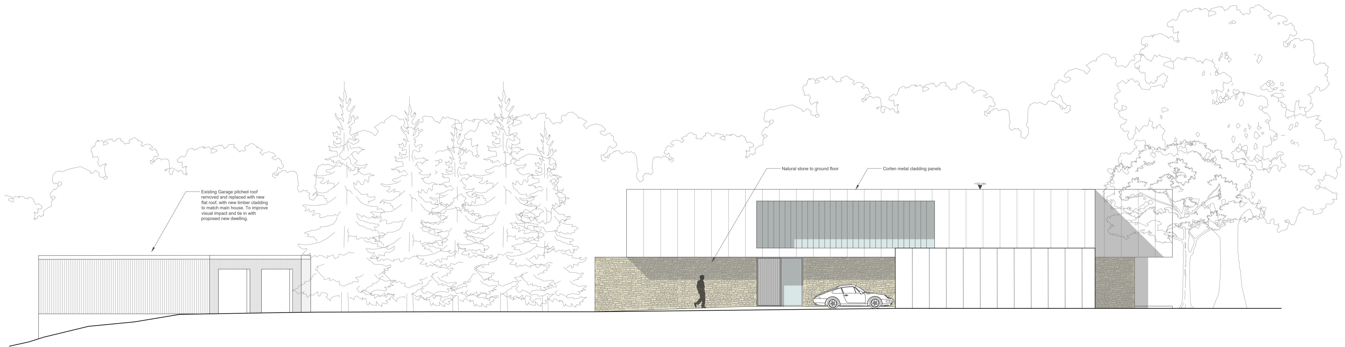
Proposed North Elevation
