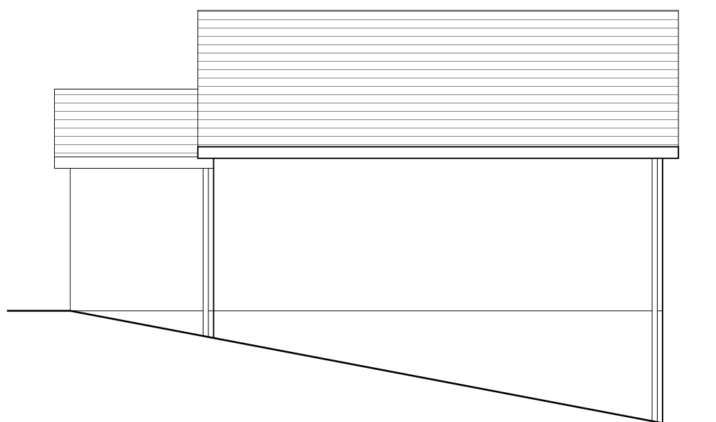
South-West Elevation
