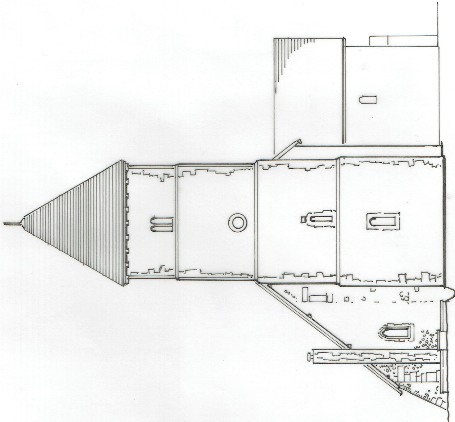
WEST ELEVATION AS EXISTING
