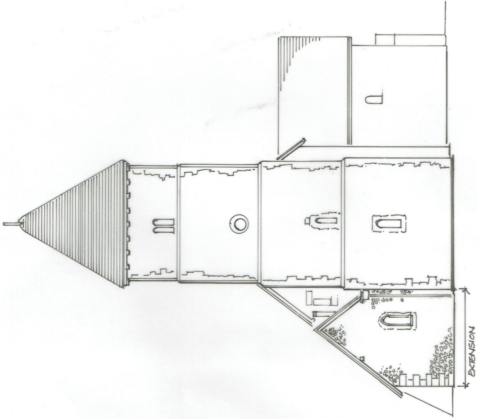
WEST ELEVATION AS PROPOSED
