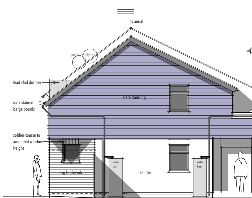
PROPOSED SOUTH (FORECOURT) ELEVATION
