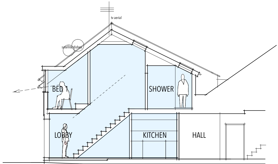
PROPOSED SECTION A-A (WEST - EAST)
