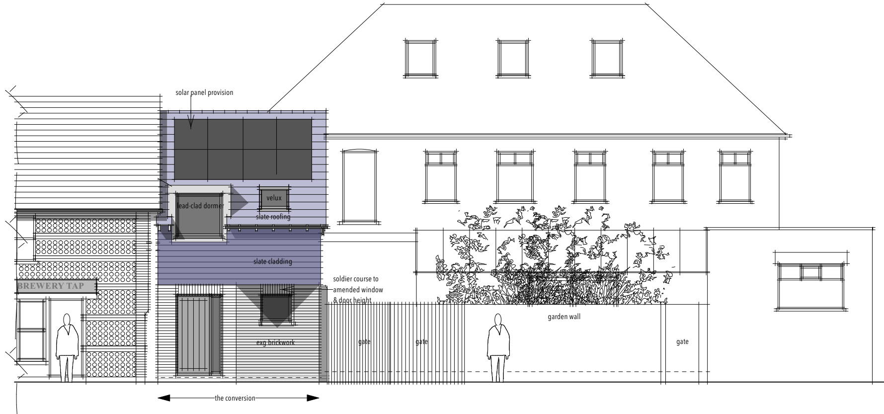
PROPOSED WEST (FRONT) ELEVATION
