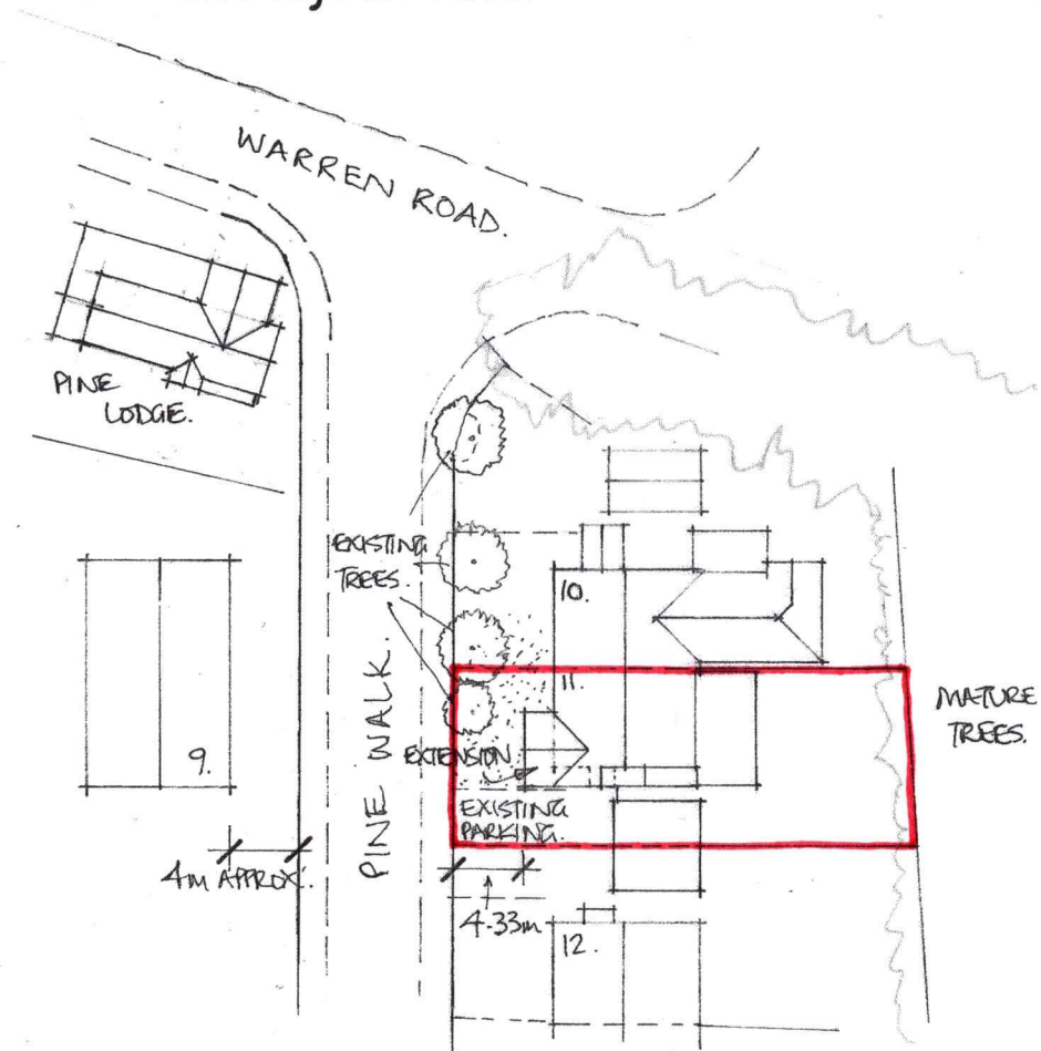
site layout. 1:500.
