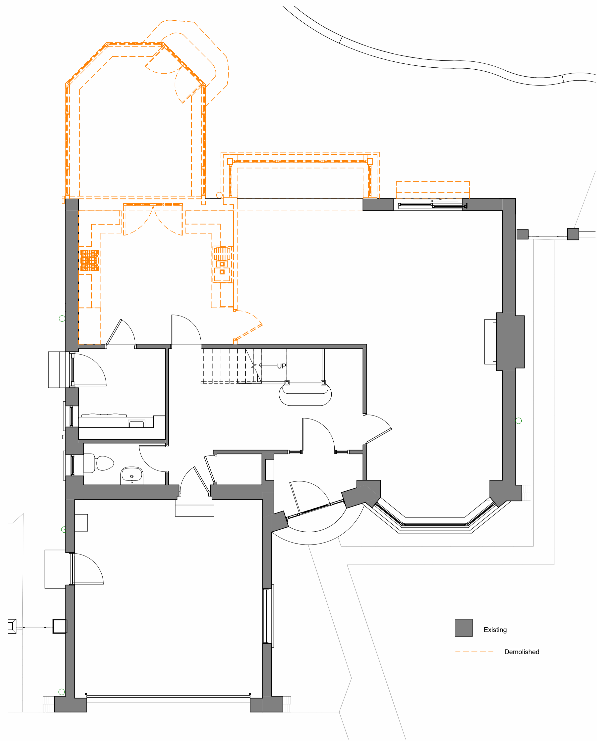
Ground Floor Plan - Removals 1 : 50
