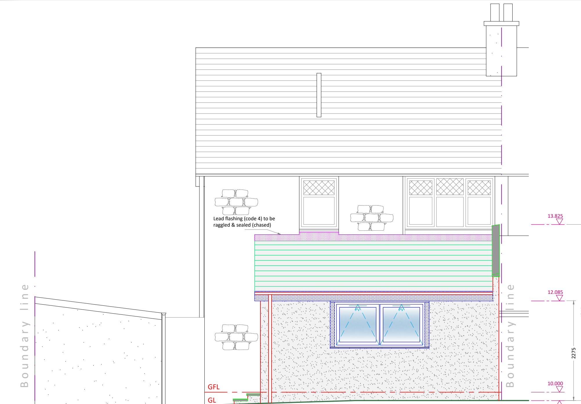
Proposed South - East Elevation(1:50)
