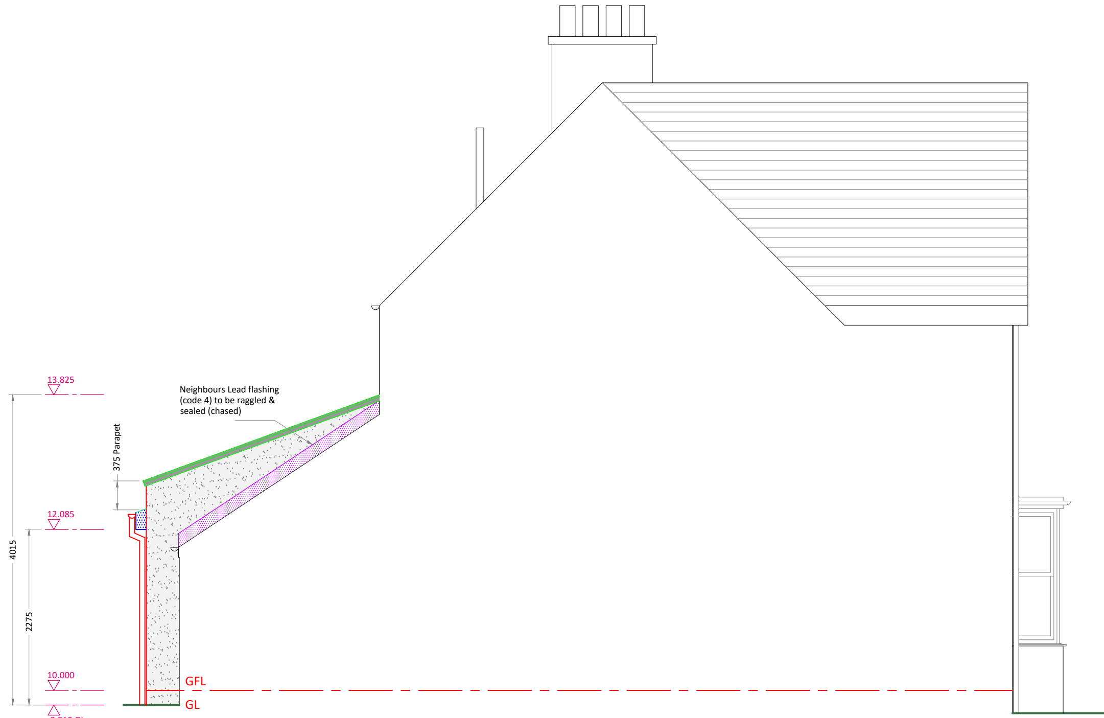
Proposed North - East Elevation (1:50)
