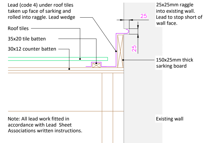
Raggle Details - Tiled Roof (1:10)
