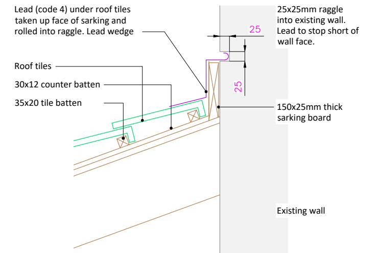
Raggle Details - Tiled Roof (1:10)
