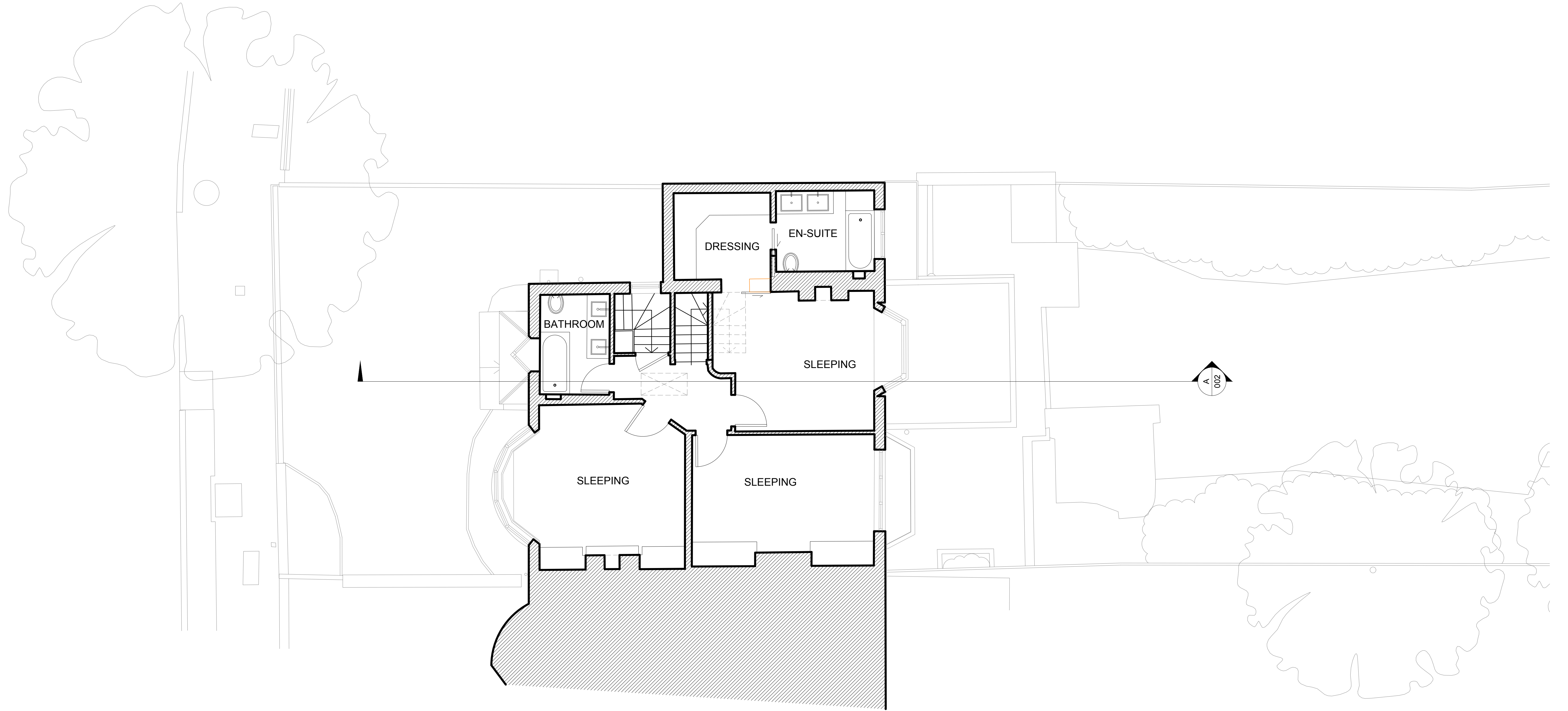
01 008 PROPOSED FIRST FLOOR PLAN
