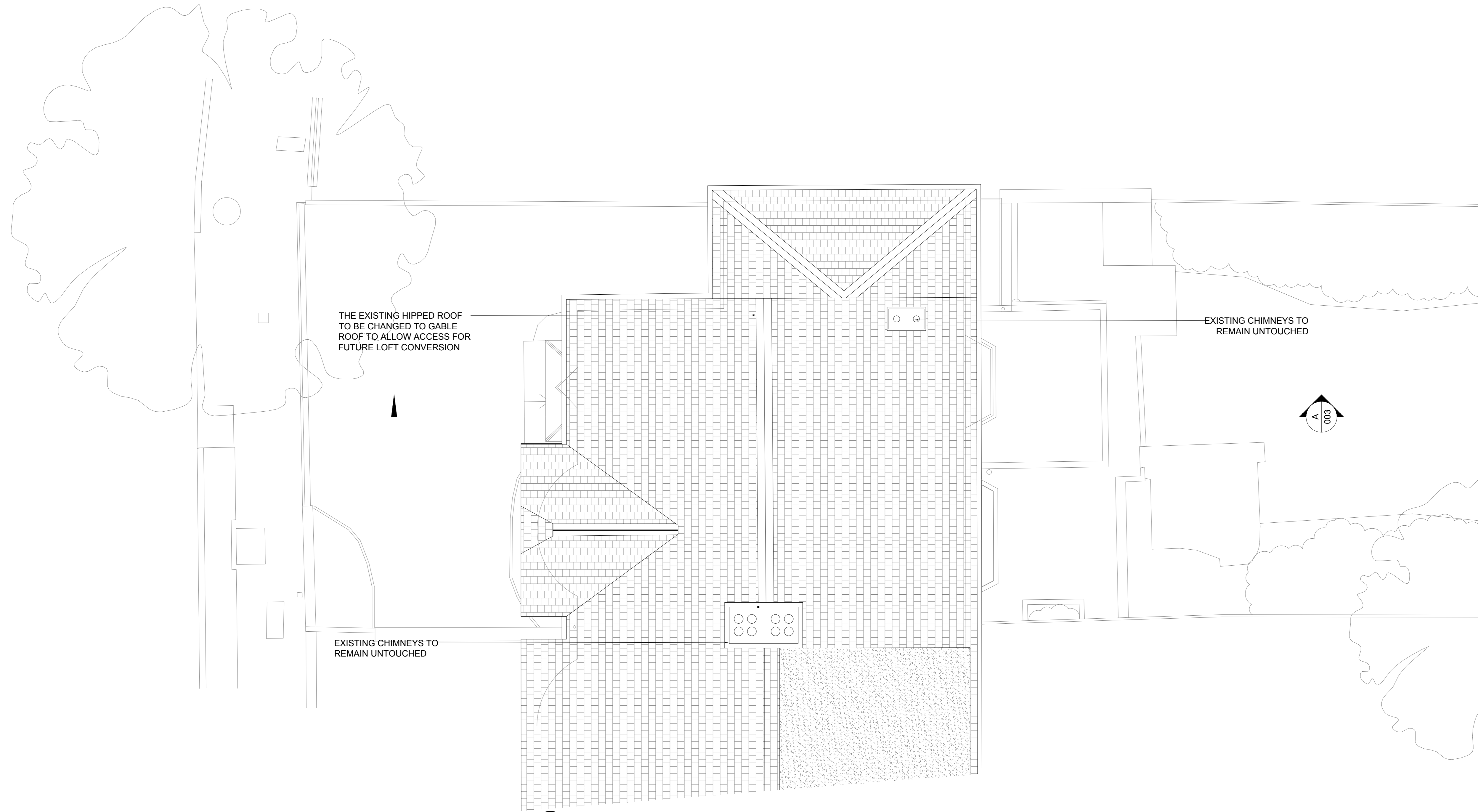
01 010A PROPOSED ROOF PLAN
