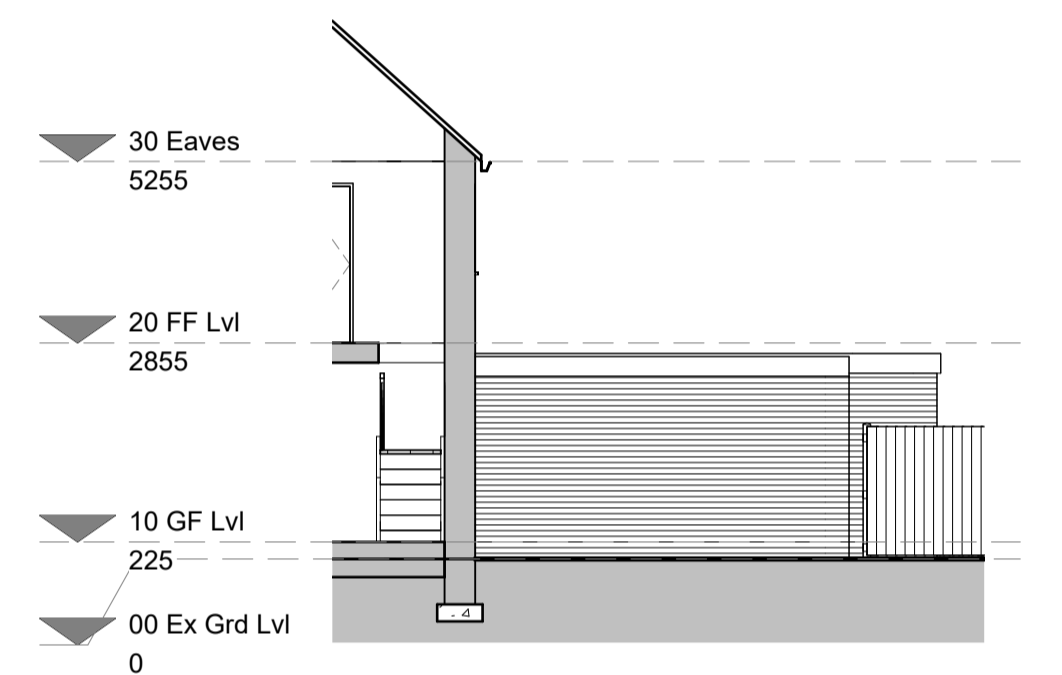
East Elevation 1 : 100
