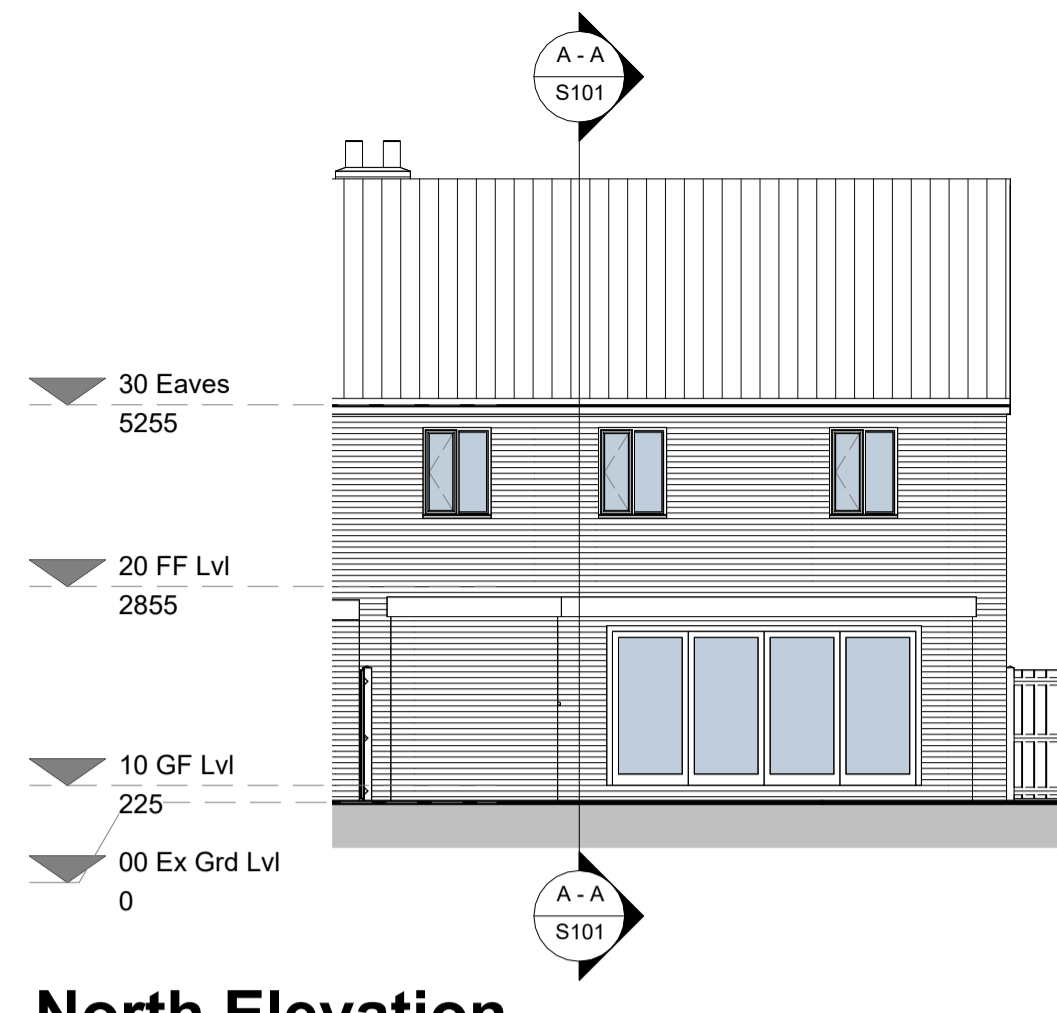
North Elevation 1 : 100
