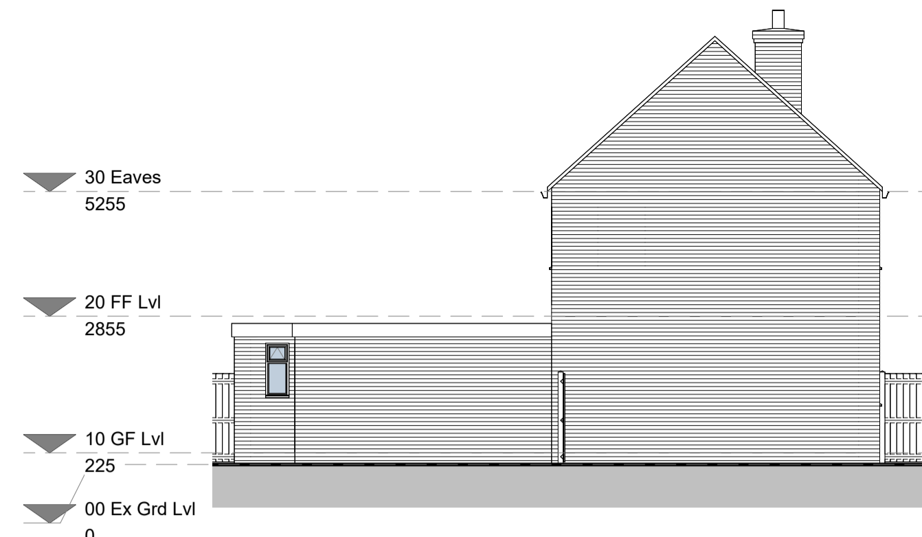
East Elevation 1 : 100
