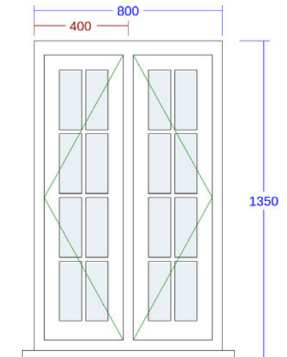
6. Flush Casement Window (Bedroom 1)
