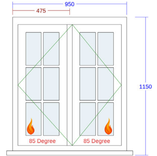
9. Flush Casement Window (Bedroom 2 )
