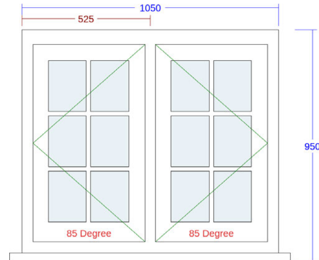
5. Flush Casement Window (Landing)
