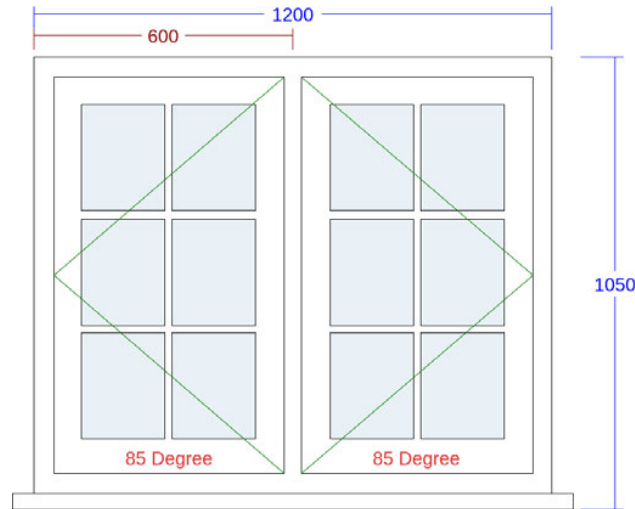
2. Flush Casement Window (Kitchen)
