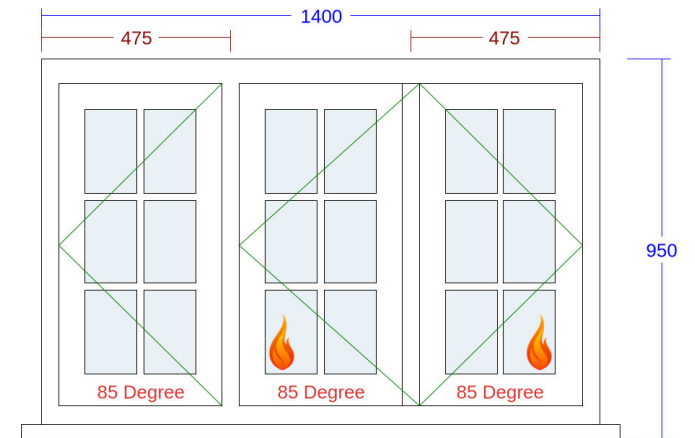
12. Flush Casement Window (Bedroom 3 )
