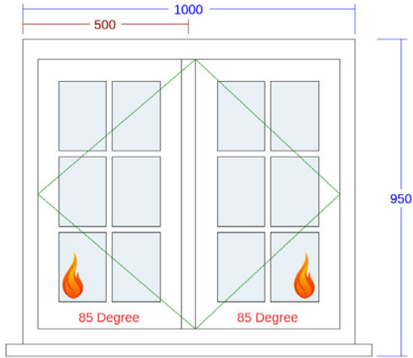
7. Flush Casement Window (Bedroom 1 )
