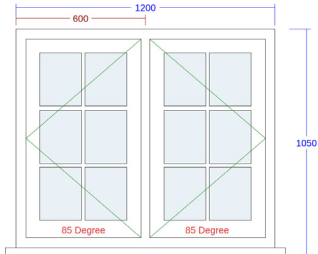
4. Flush Casement Window (Kitchen)
