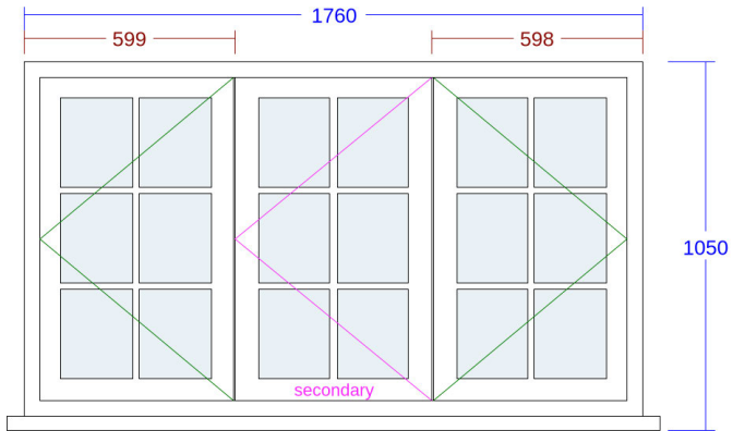
1. Conventional Cottage Window (Lounge)
