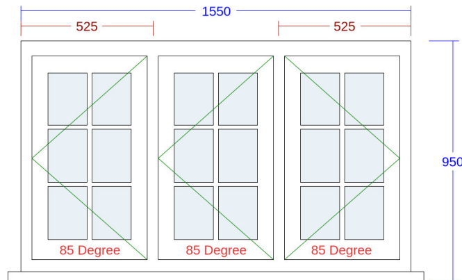
11. Flush Casement Window (Bathroom )
