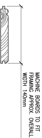
SECTION DETAIL THROUGH ALL GATE BOARDS EXCEPT THE RIGHT HAND BOARD OF EACH GATE (WHEN VIEWED FROM MARKET PLACE-SEE DETAIL BELOW) SCALE: 1:5
