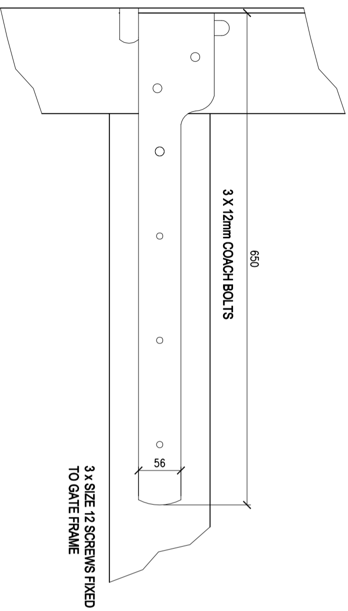
ELEVATION DETAIL SHOWING GATE HINGE & PIN SCALE: 1:5
