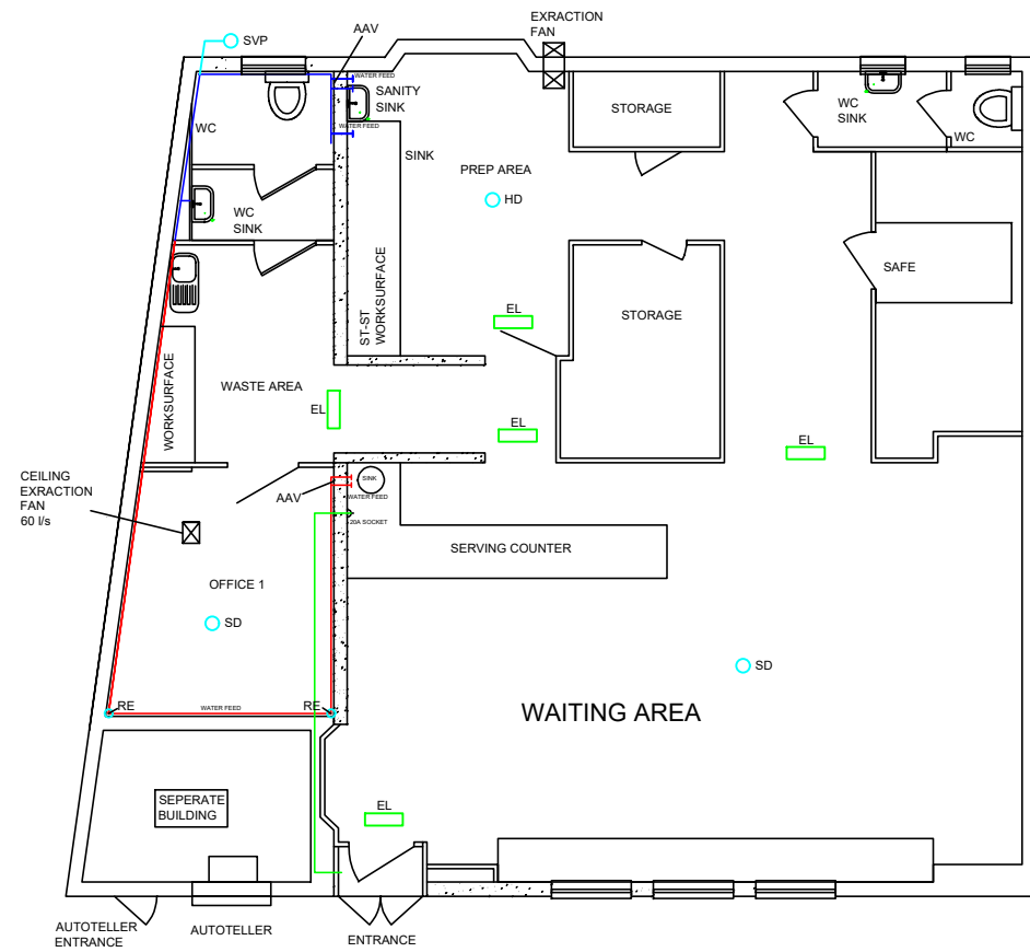
PROPOSED GROUND FLOOR LAYOUT 1:100
