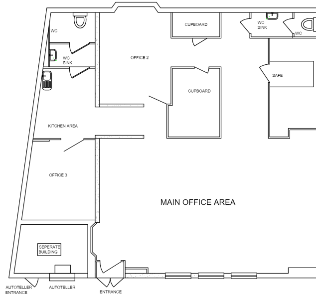
EXISTING GROUND FLOOR LAYOUT 1:100
