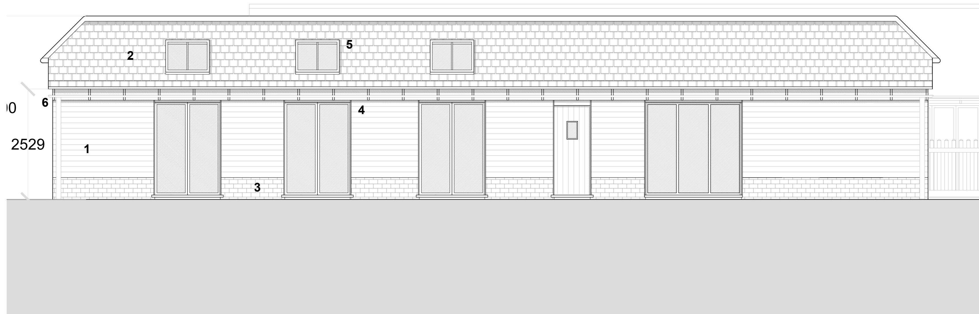
Proposed East Elevation: Barn 3 | 1:50
