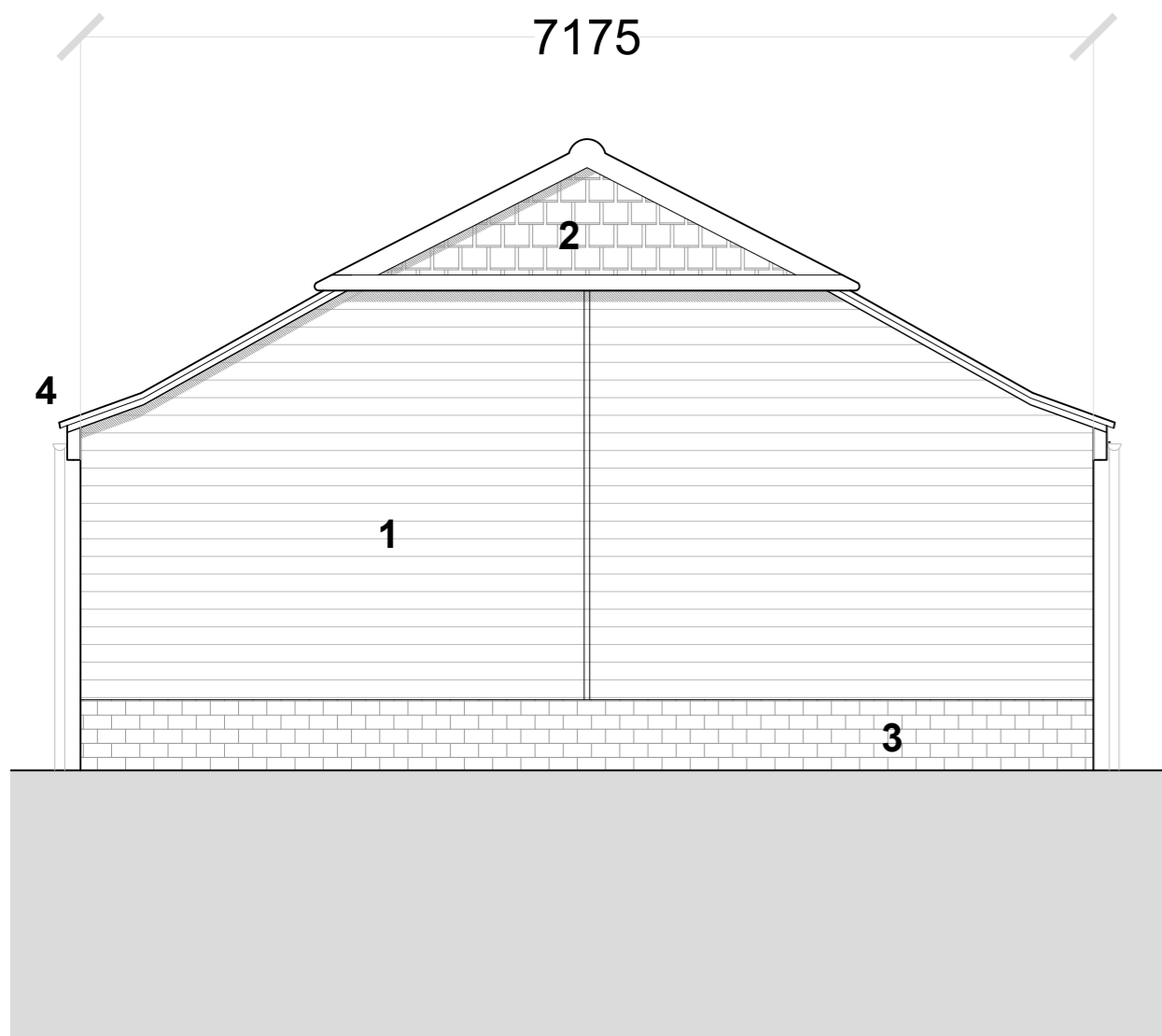
Proposed North Elevation: Barn 1 | 1:50
