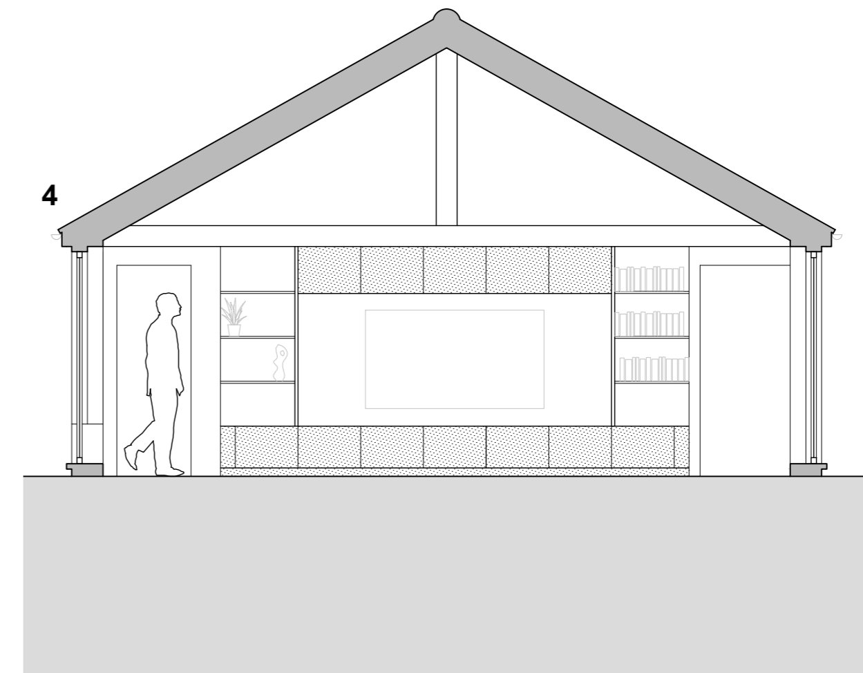
Proposed Section AA: Barn 1 | 1:50
