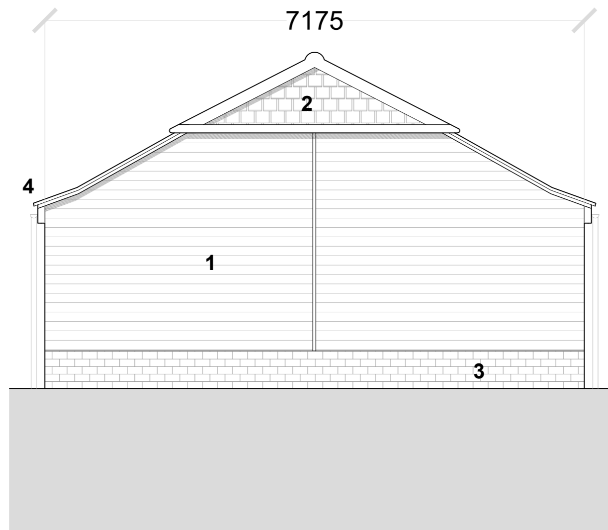
Proposed South Elevation: Barn 1 | 1:50
