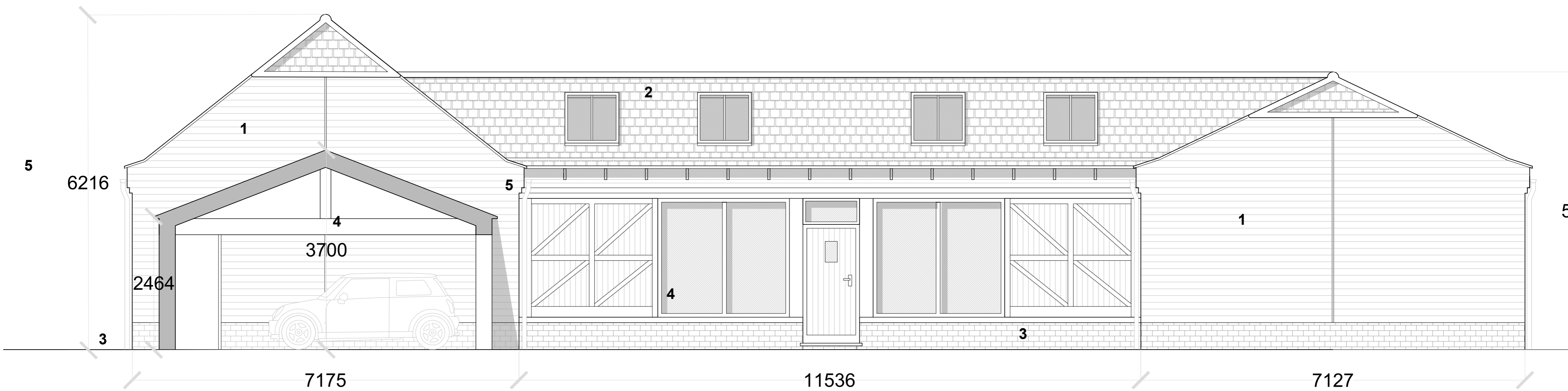
Proposed South Elevation: Barn 2 | 1:50
