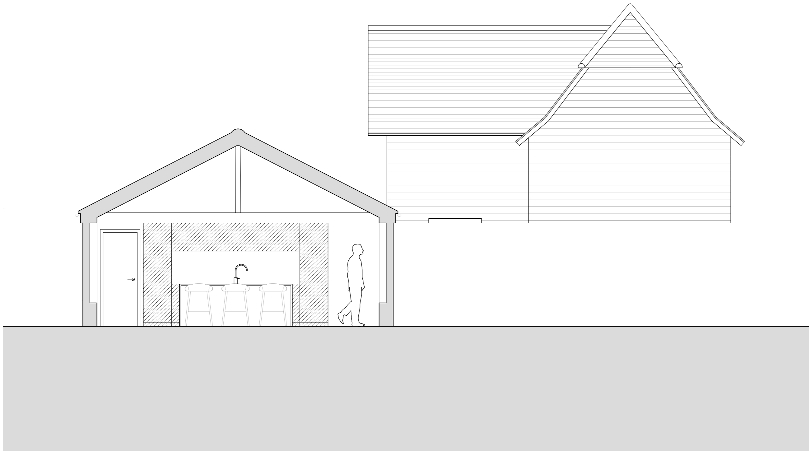
Proposed Section BB Barn 3 | 1:50
