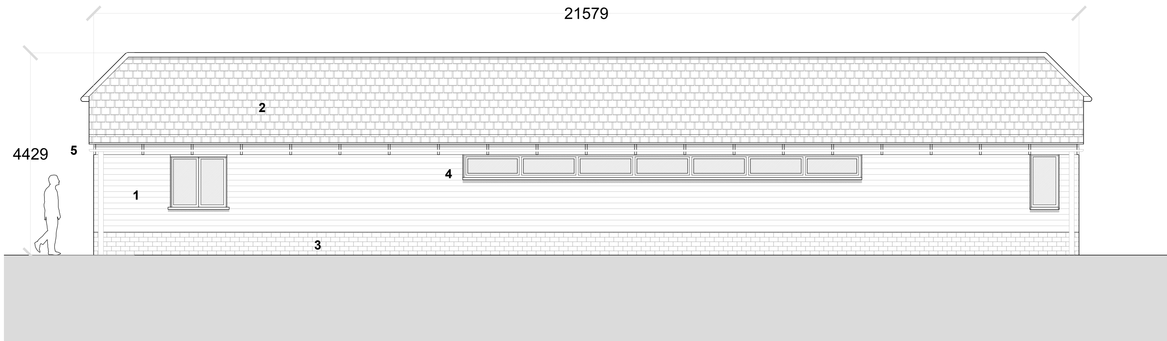
Proposed West Elevation: Barn 1 | 1:50
