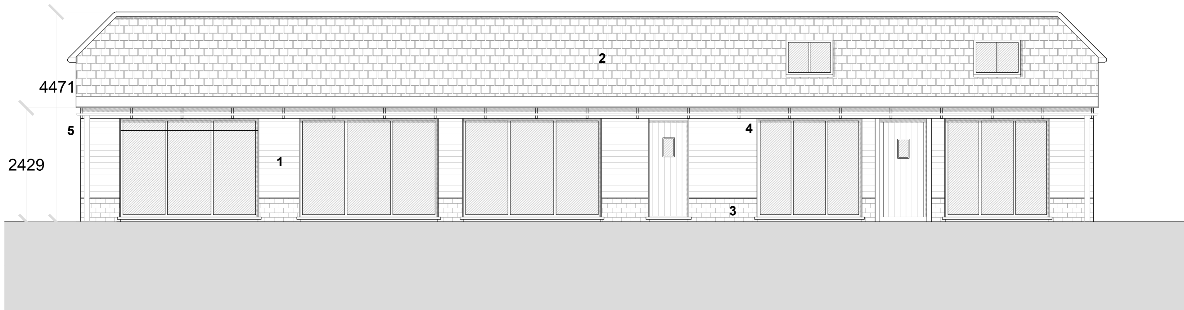
Proposed Front Elevation: Barn 1 | 1:50
