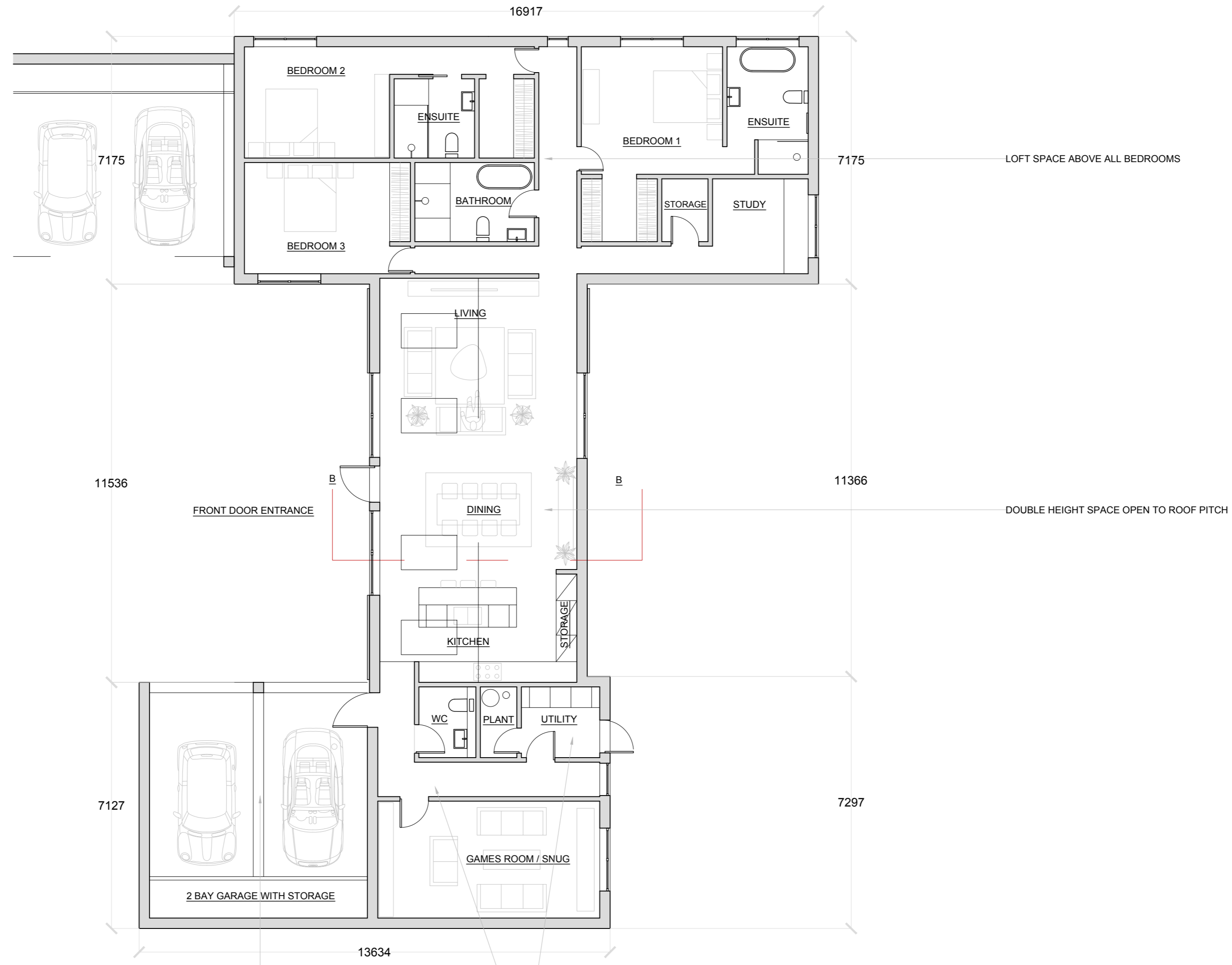
Proposed Ground Floor Plan: Barn 2 | 1:100
