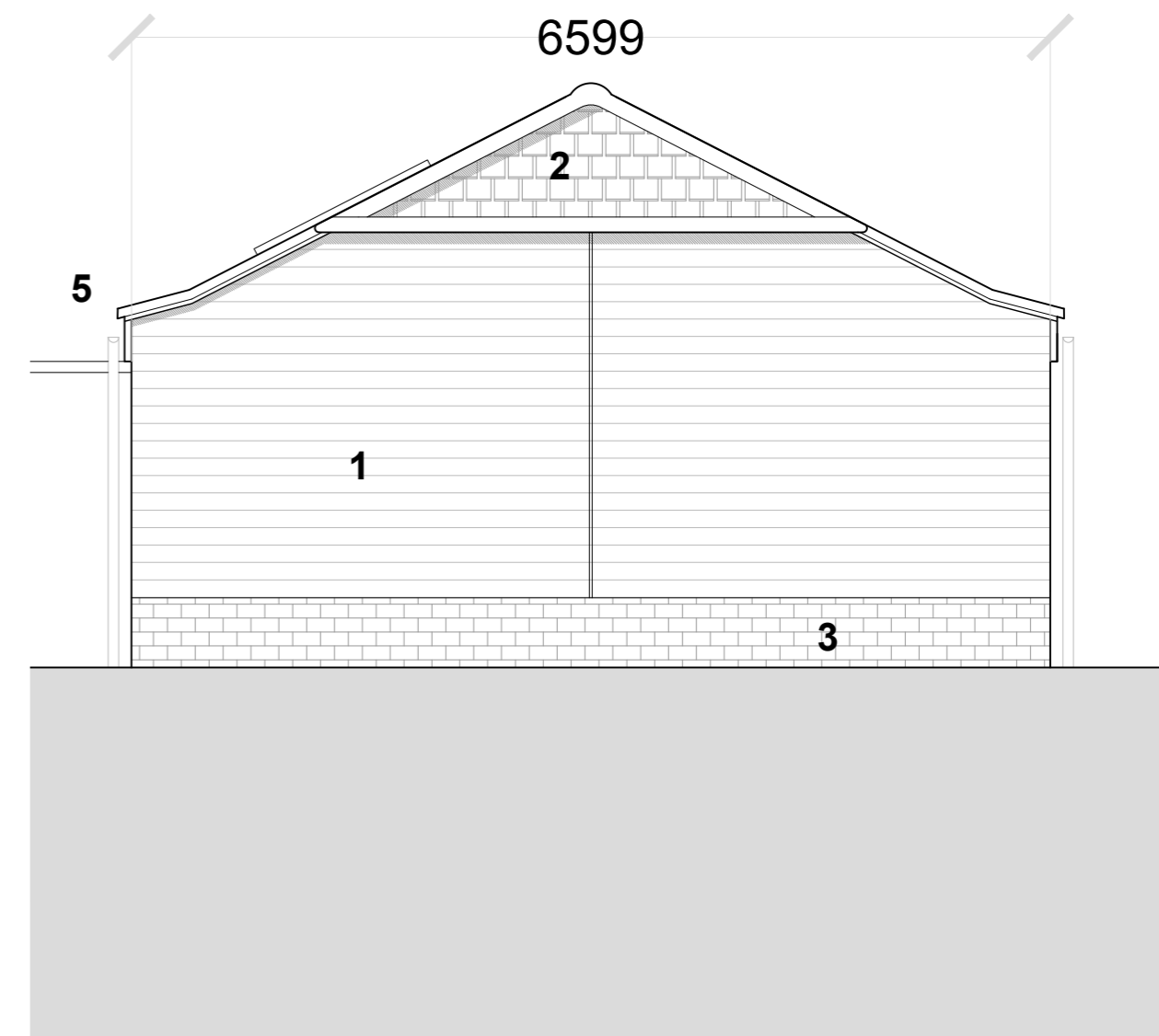
Proposed South Elevation: Barn 3 | 1:50
