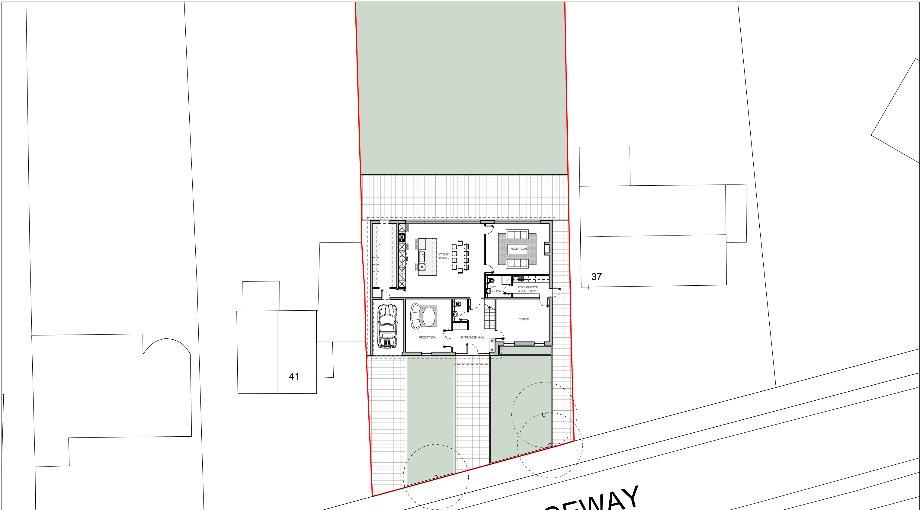
I Proposed Ground Floor Plan Scale: 1:200
