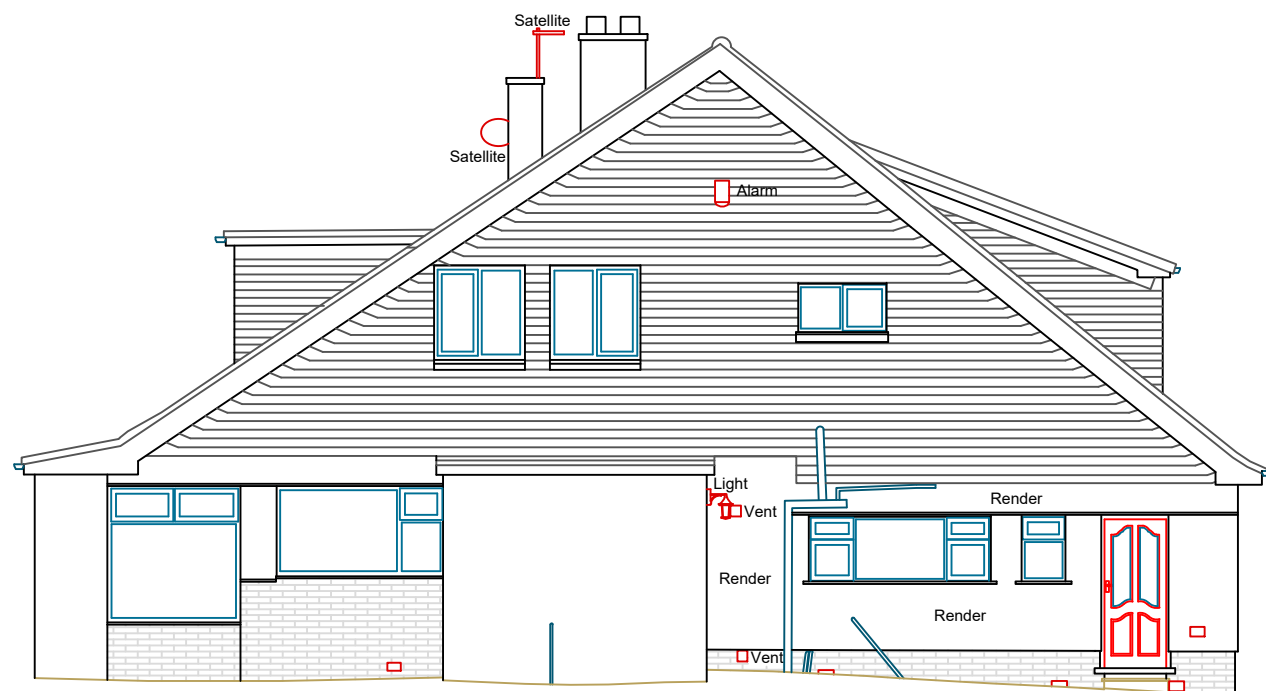
Elevation C
