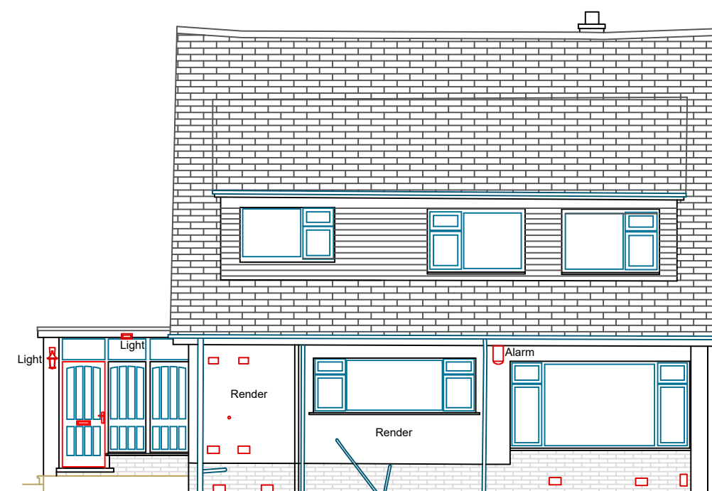
Elevation D
