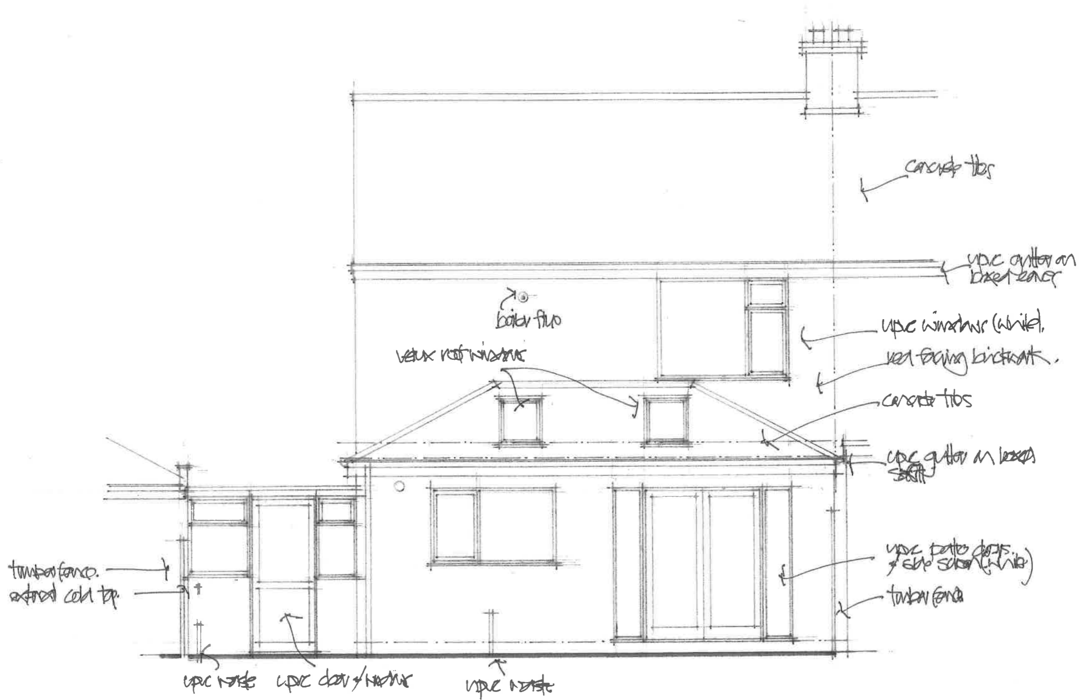
Rear Elevation
