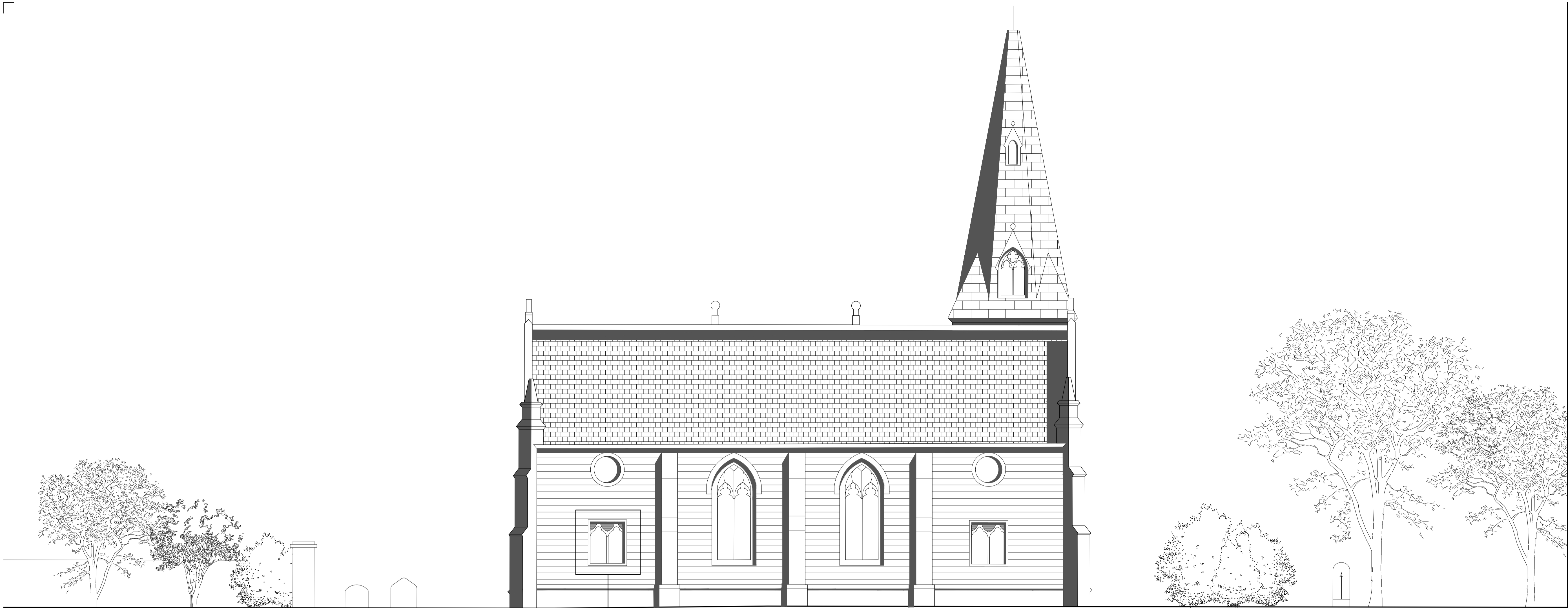
PROPOSED ELEVATION C SCALE 1:100 @ A1
