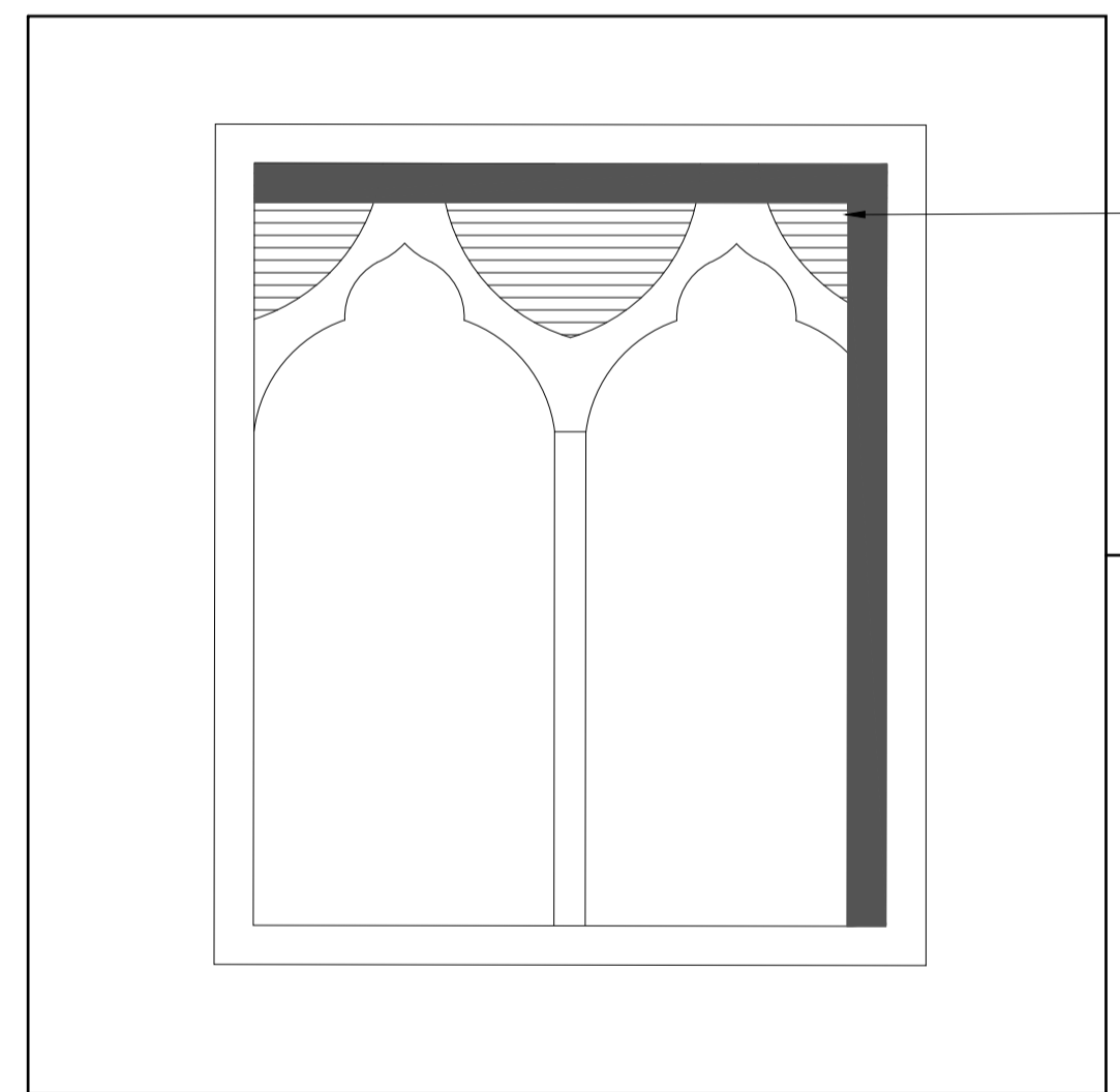
WINDOW ALTERATION SCALE 1:20 @ A1
