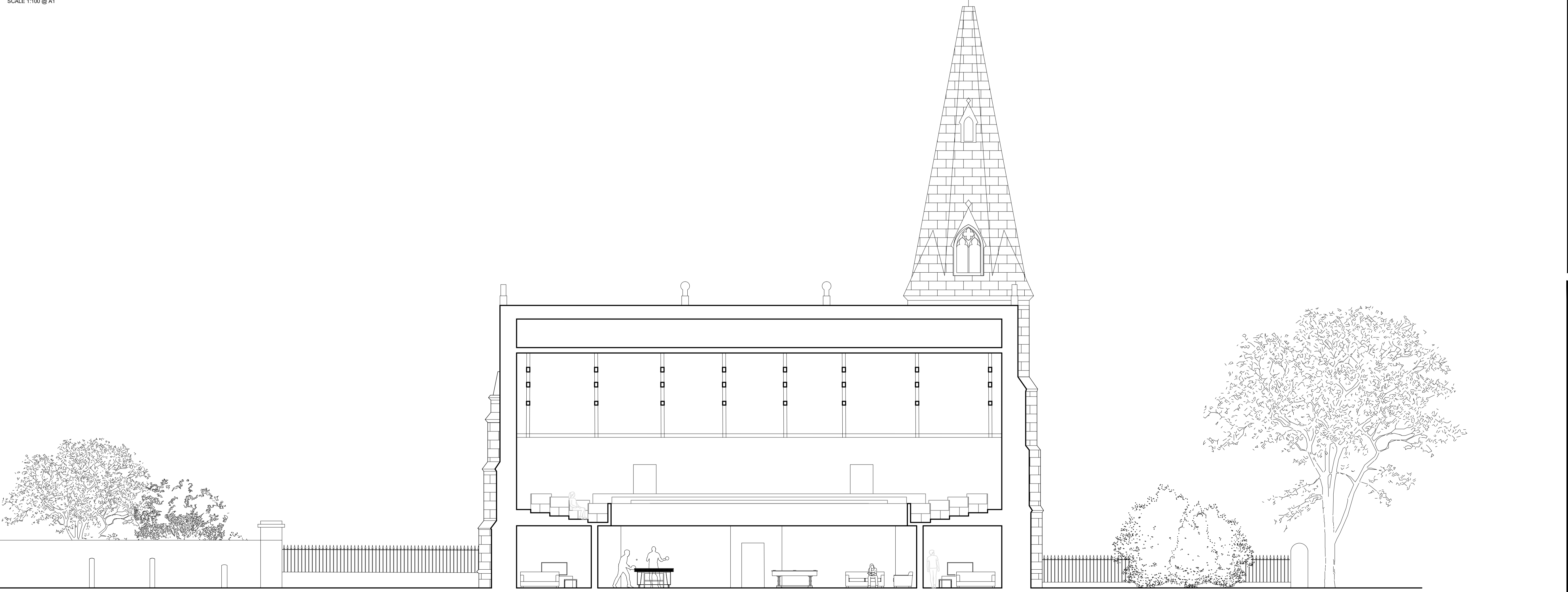
PROPOSED SECTION B-B SCALE 1:100 @ A1
