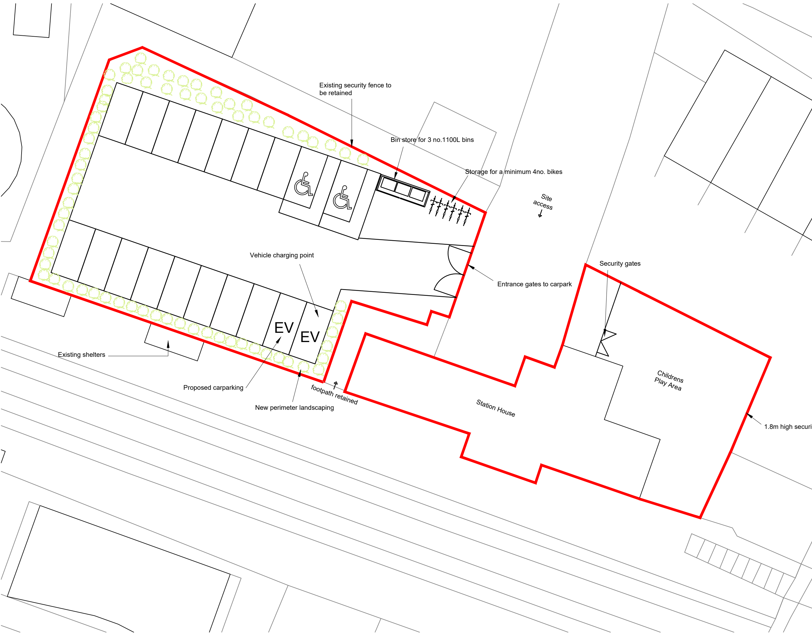
Block Plan Scale 1:200
