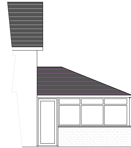
Side 2 Elevation Proposed
