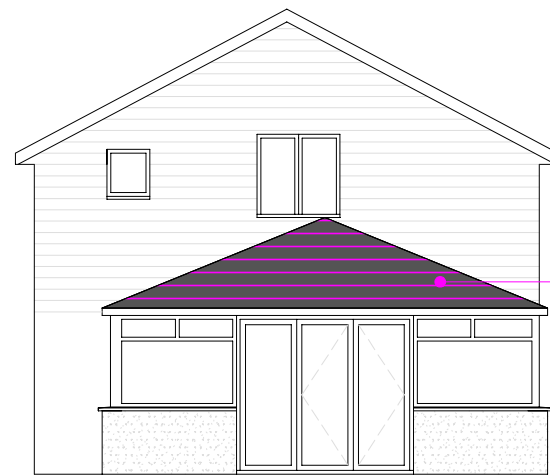
Front Elevation Proposed
