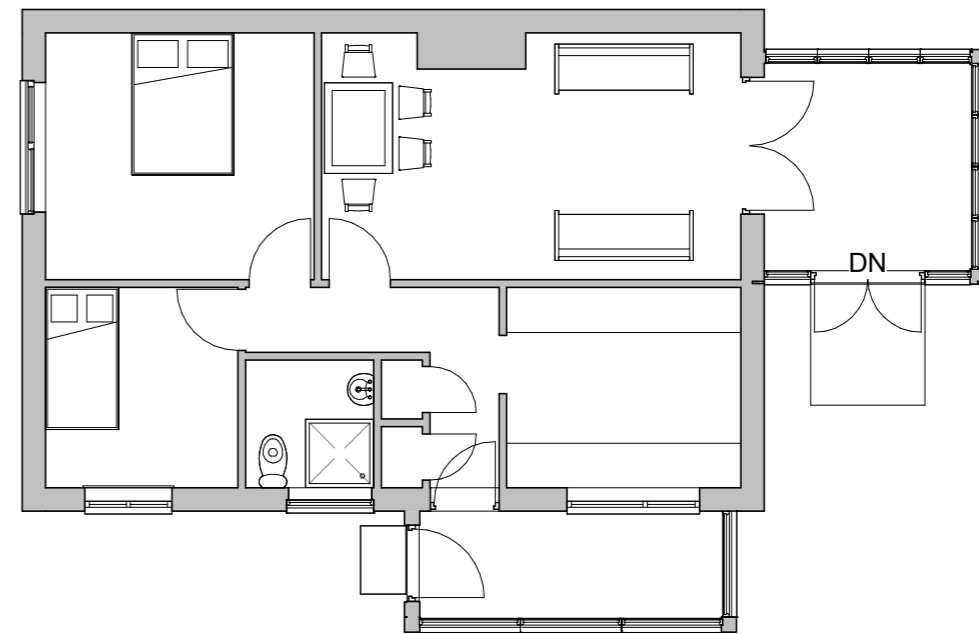
5 Ground Floor 1 : 100
