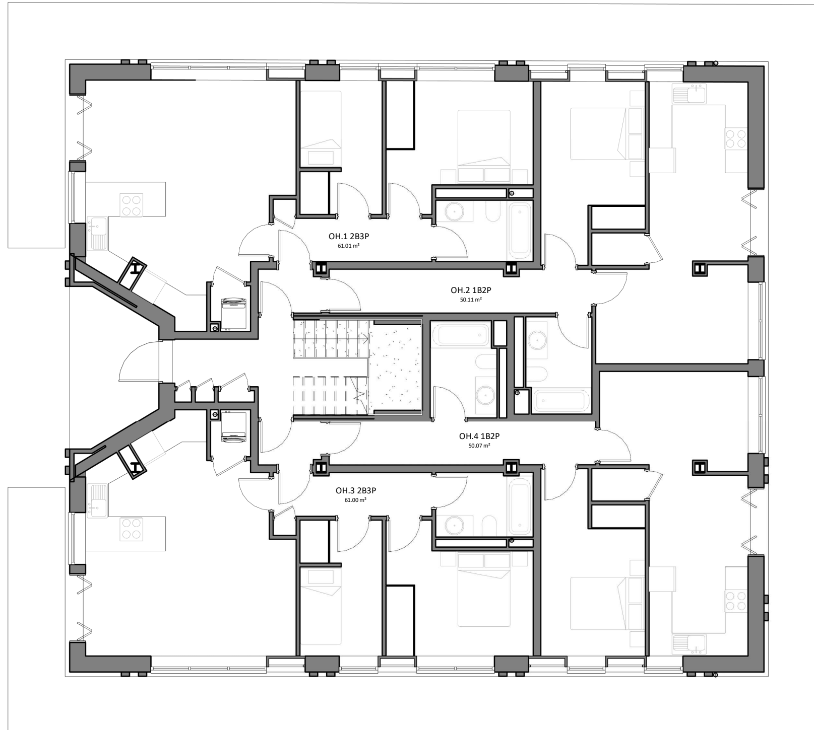
1 GA - 00_Ground OCE100 Scale - 1 : 100
