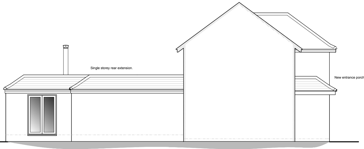
North Elevation | sectional proposed
