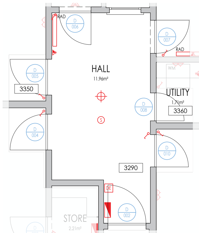
1_HALL PLAN 1:50 @ A3
