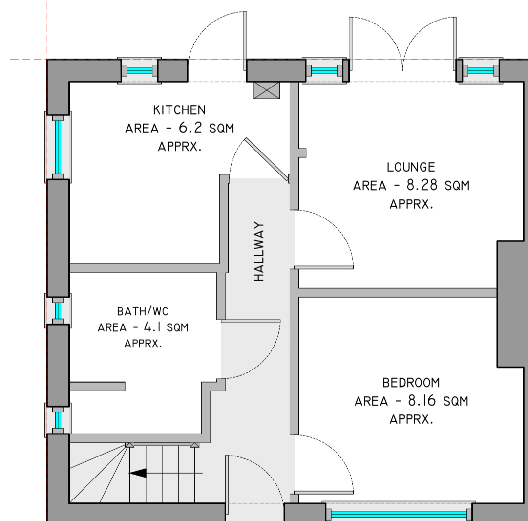
GROUND FLOOR, PROPOSED PLAN, SCALE 1:50 (NO ALTERATIONS TO LAYOUT PROPOSED)
