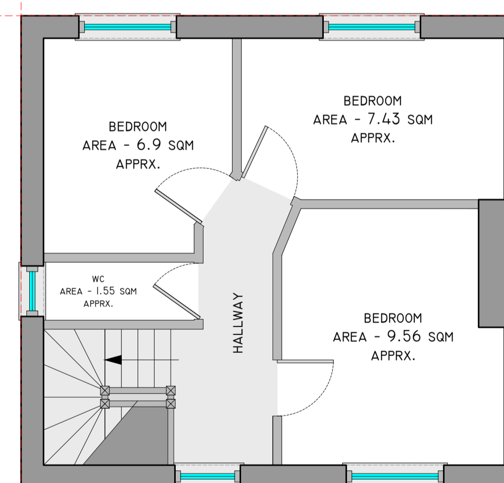
FIRST FLOOR, PROPOSED PLAN, SCALE 1:50 (NO ALTERATIONS TO LAYOUT PROPOSED)
