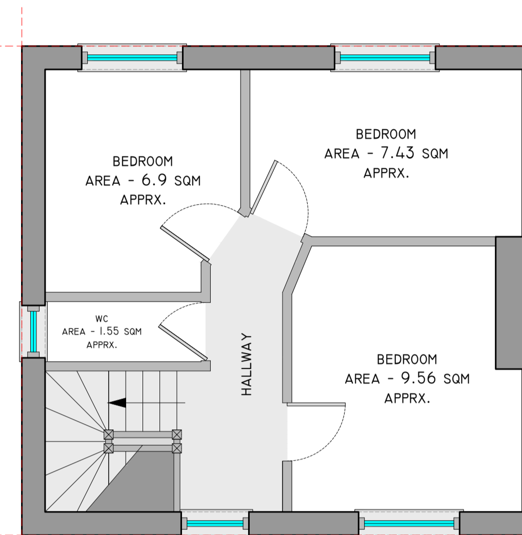
FIRST FLOOR, EXISTING PLAN, SCALE 1:50
