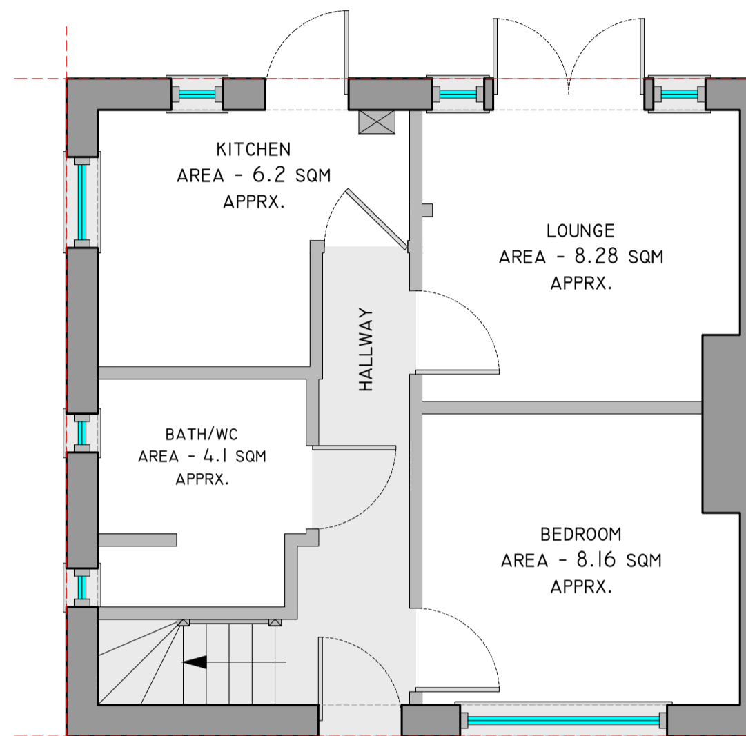
GROUND FLOOR, EXISTING PLAN, SCALE 1:50
