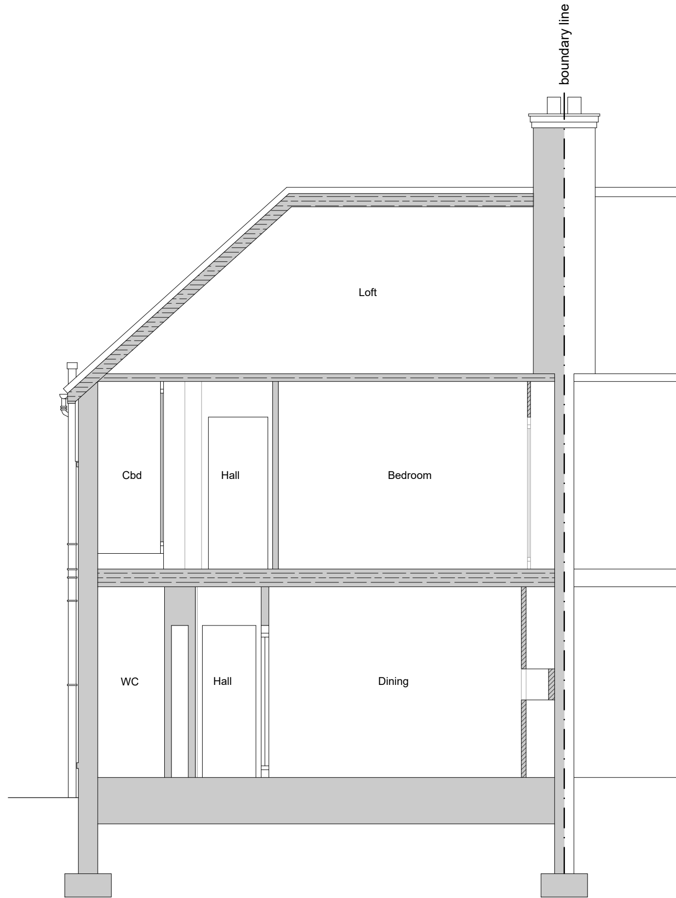
Existing Section A-A Scale - 1:50@A3
