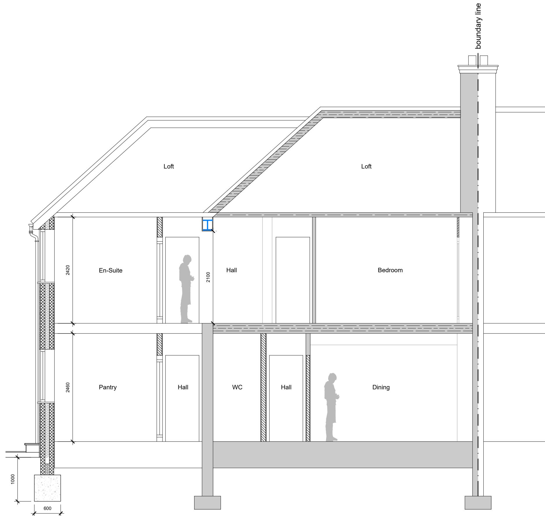
Proposed Section A-A Scale - 1:50@A3
