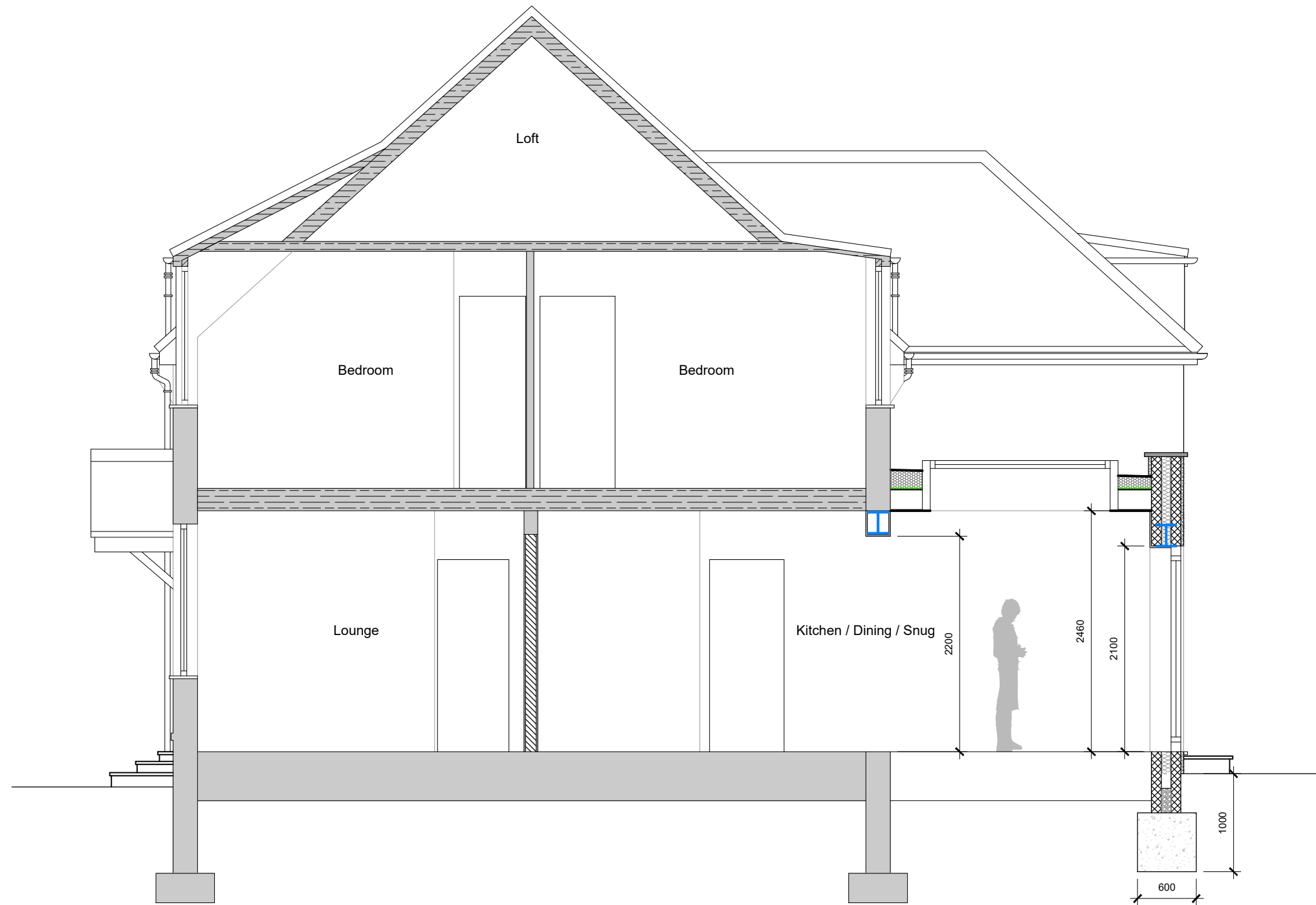
Proposed Section B-B Scale - 1:50@A3
