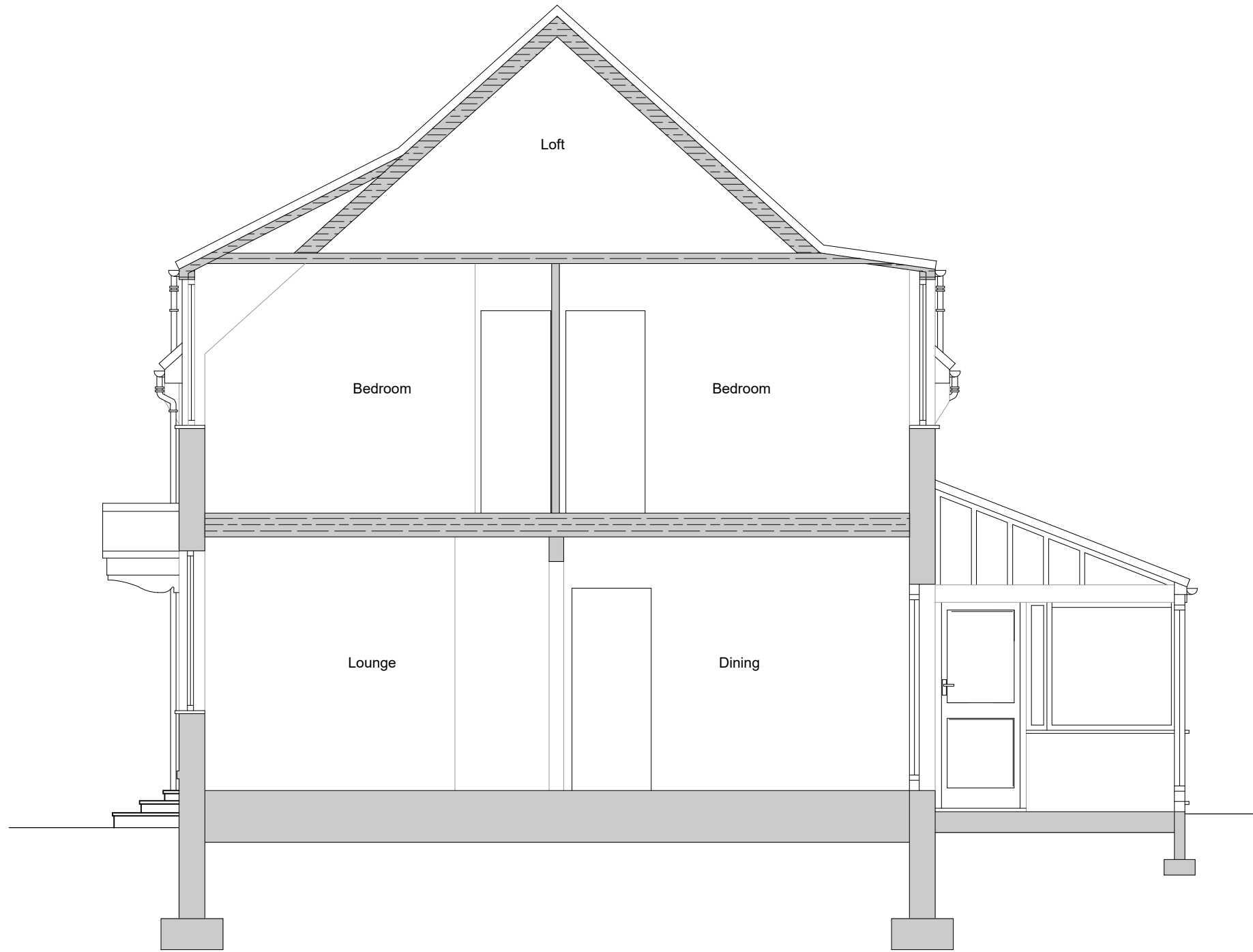
Existing Section B-B Scale - 1:50@A3
