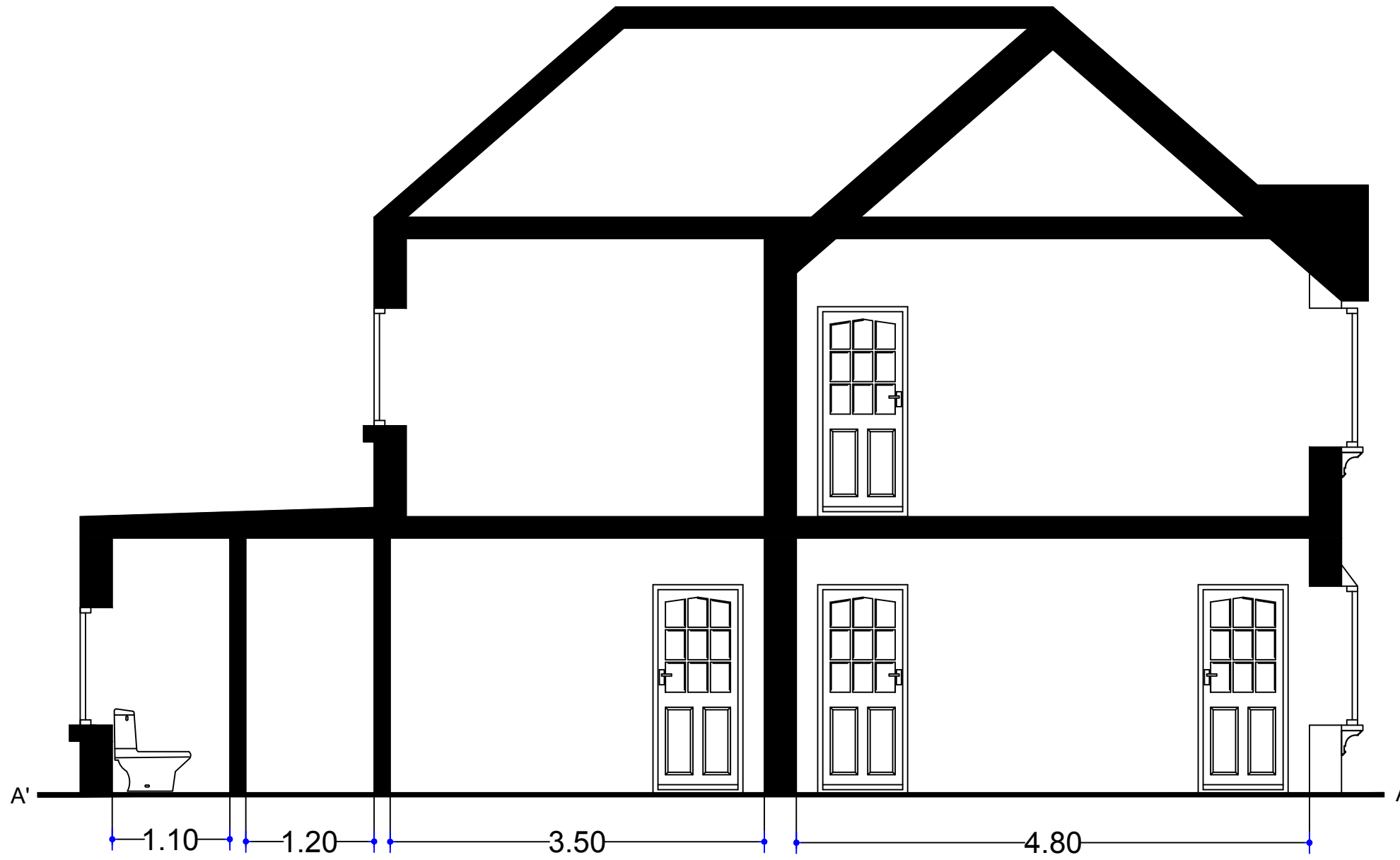
Proposed Cross-Sectional A-A' View
