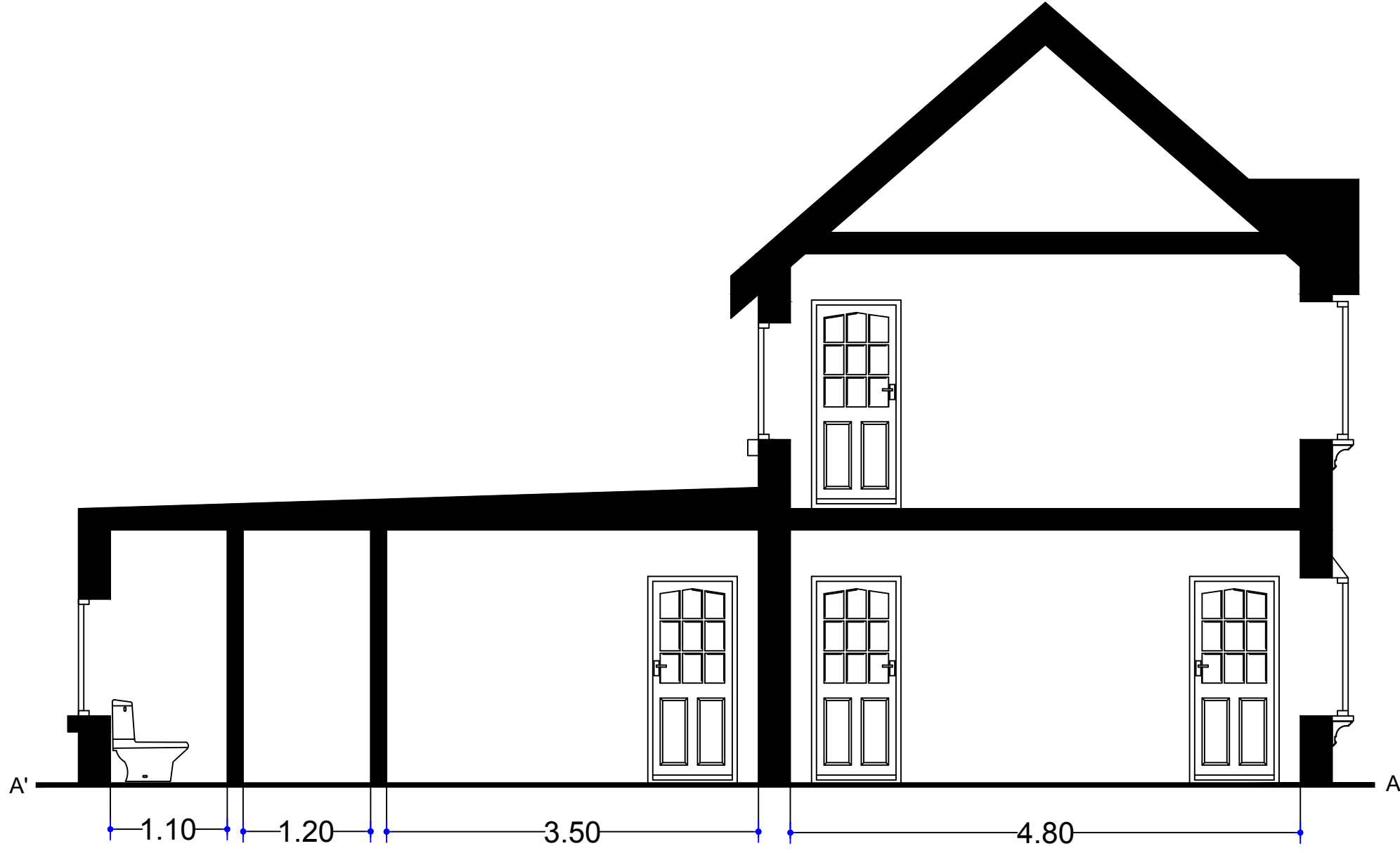
Existing Cross-Sectional A-A' View
