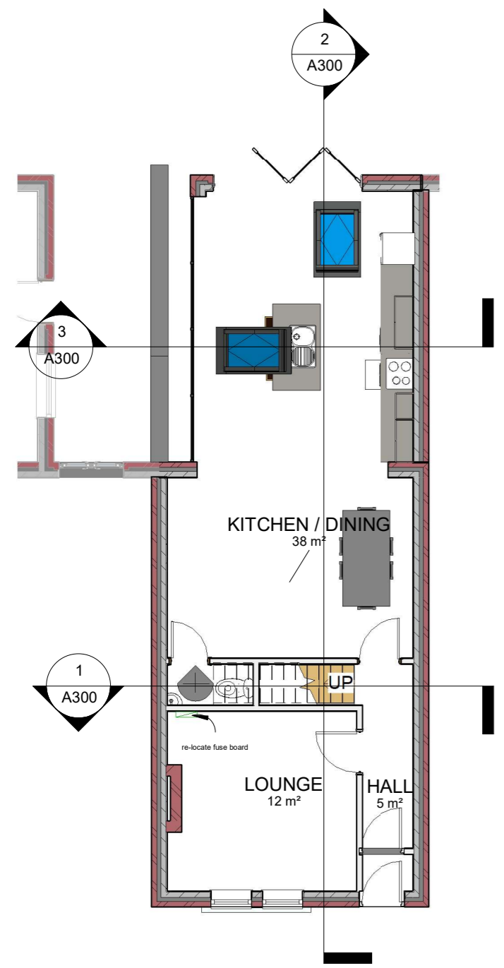
② GF PROPOSED 1 : 100
