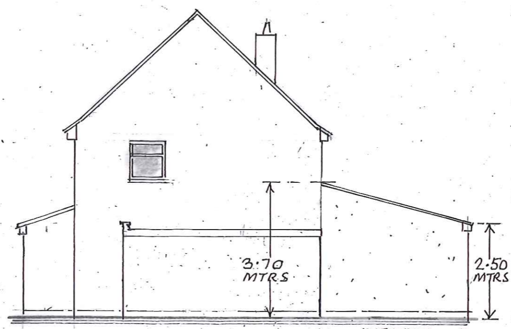
SIDE EL.
